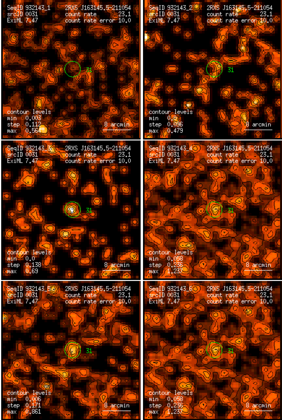
Figure 31: RASS 932143: detection 0031: band rate images, Gaussian filter: (1) PSPC channels 11 – 41, (2) 52 – 90, (3) 91 – 201, (4) 11 – 235, (5) 52 – 201, (6) 11 – 201. Broad band rates in counts/ks. Band rate contour levels in counts/ks/arcmin 2 .
