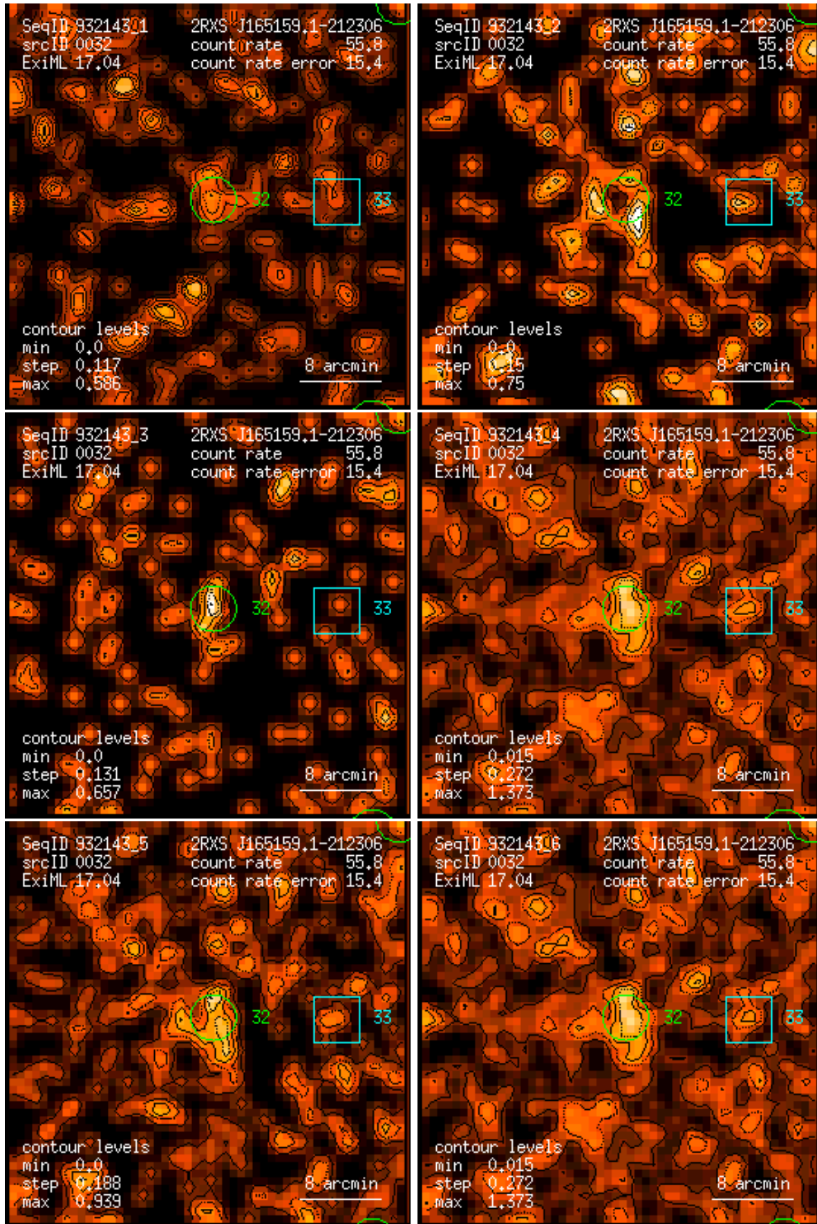
Figure 32: RASS 932143: detection 0032: band rate images, Gaussian filter: (1) PSPC channels 11 – 41, (2) 52 – 90, (3) 91 – 201, (4) 11 – 235, (5) 52 – 201, (6) 11 – 201. Broad band rates in counts/ks. Band rate contour levels in counts/ks/arcmin 2 .
