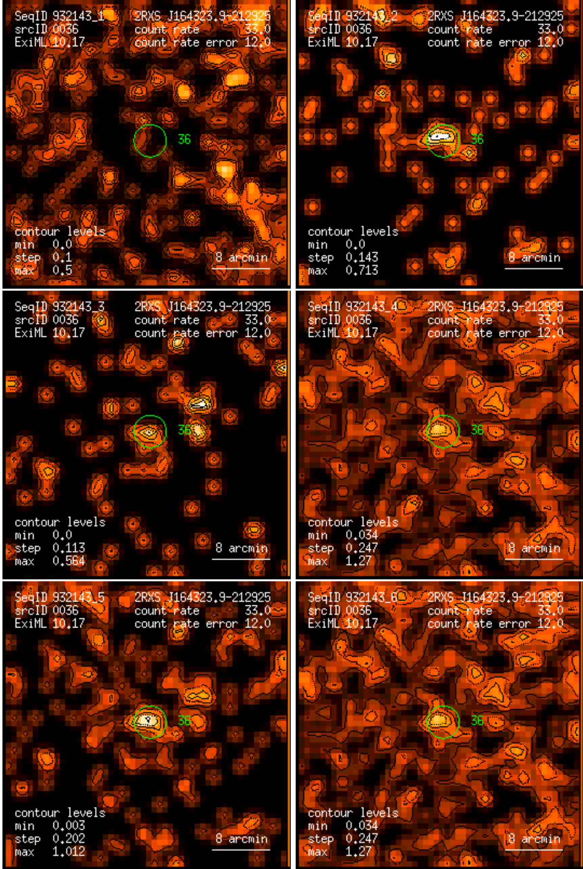
Figure 36: RASS 932143: detection 0036: band rate images, Gaussian filter: (1) PSPC channels 11 – 41, (2) 52 – 90, (3) 91 – 201, (4) 11 – 235, (5) 52 – 201, (6) 11 – 201. Broad band rates in counts/ks. Band rate contour levels in counts/ks/arcmin 2 .
