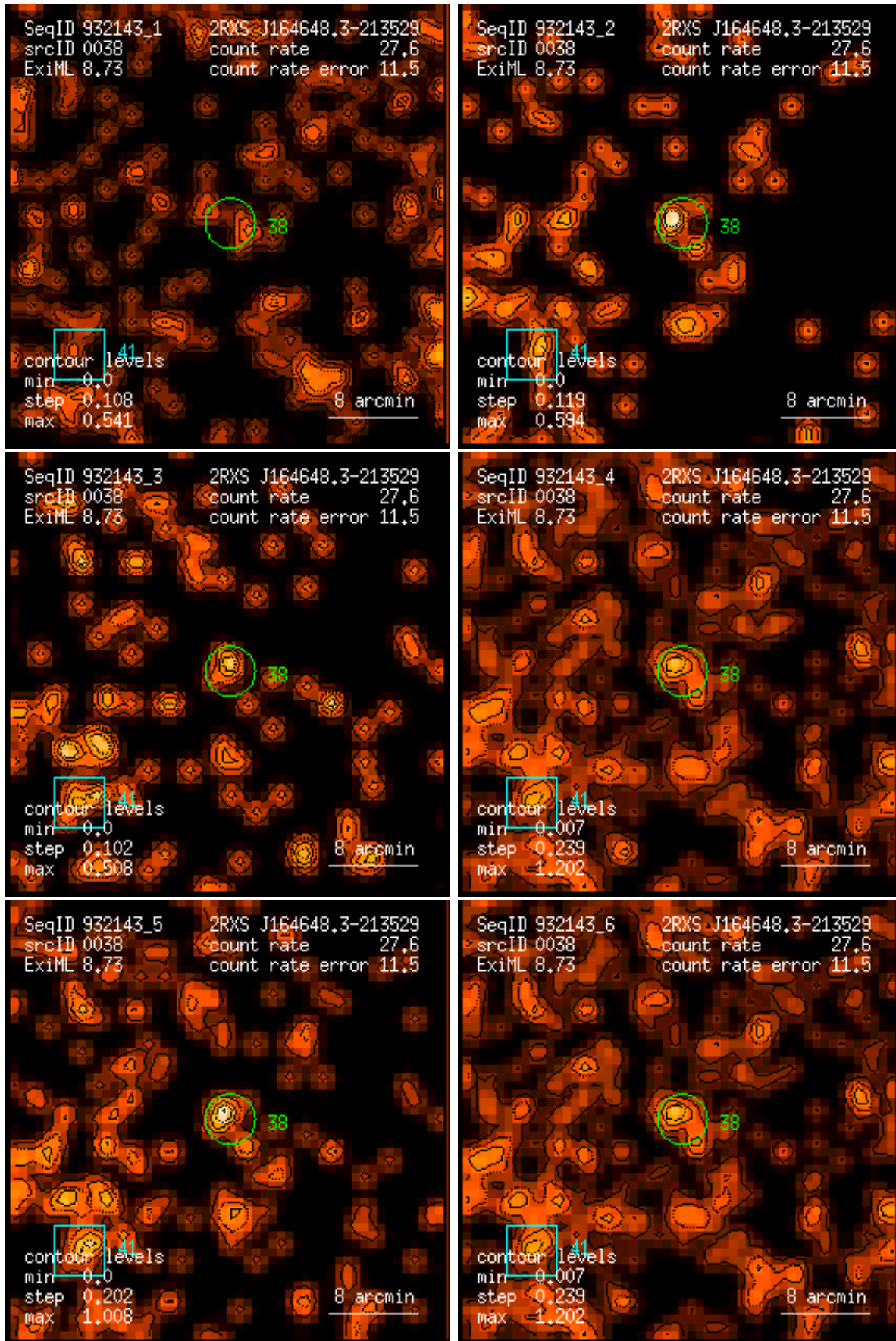
Figure 38: RASS 932143: detection 0038: band rate images, Gaussian filter: (1) PSPC channels 11 – 41, (2) 52 – 90, (3) 91 – 201, (4) 11 – 235, (5) 52 – 201, (6) 11 – 201. Broad band rates in counts/ks. Band rate contour levels in counts/ks/arcmin 2 .
