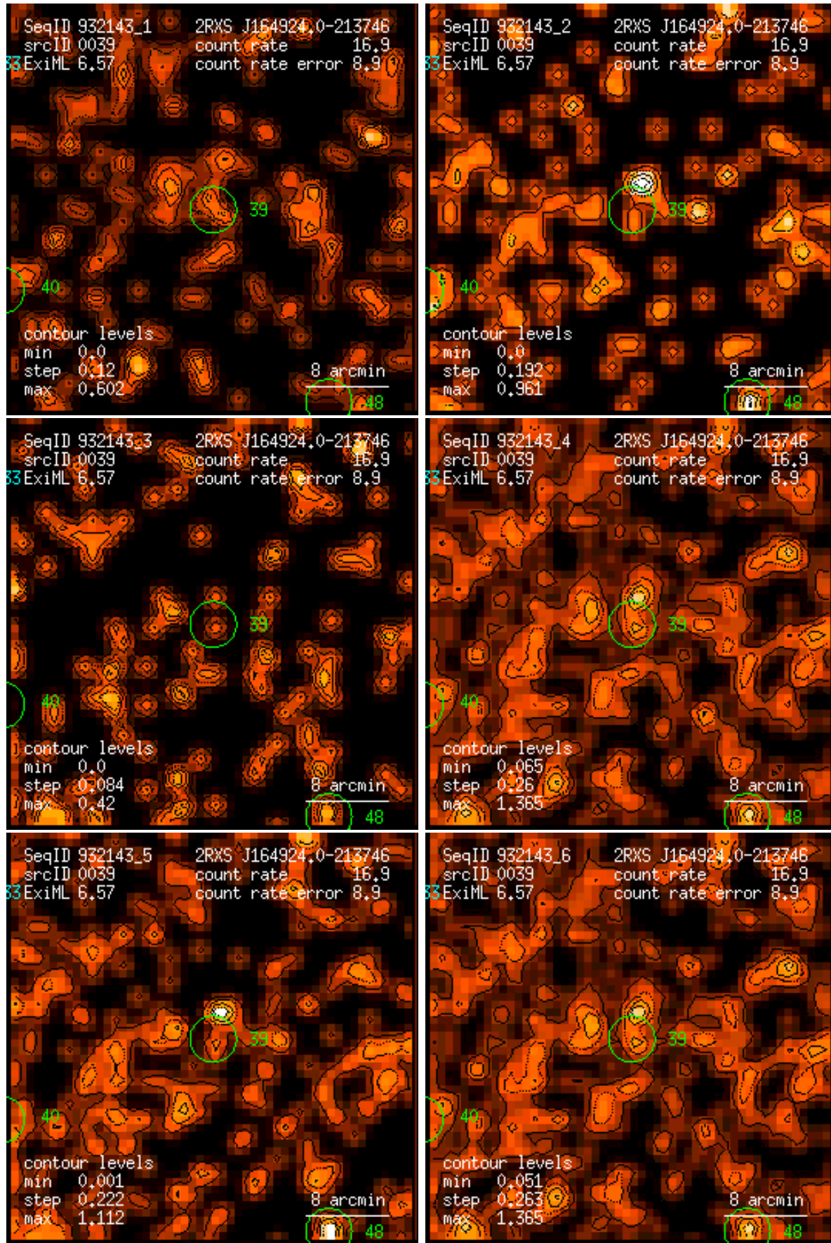
Figure 39: RASS 932143: detection 0039: band rate images, Gaussian filter: (1) PSPC channels 11 – 41, (2) 52 – 90, (3) 91 – 201, (4) 11 – 235, (5) 52 – 201, (6) 11 – 201. Broad band rates in counts/ks. Band rate contour levels in counts/ks/arcmin 2 .
