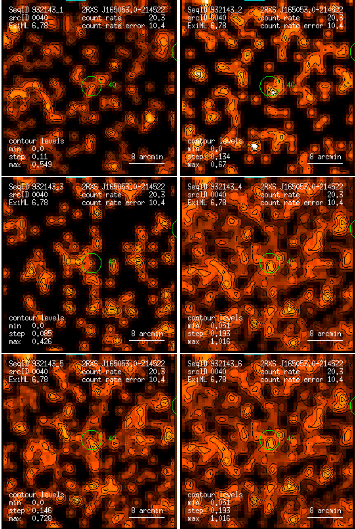
Figure 40: RASS 932143: detection 0040: band rate images, Gaussian filter: (1) PSPC channels 11 – 41, (2) 52 – 90, (3) 91 – 201, (4) 11 – 235, (5) 52 – 201, (6) 11 – 201. Broad band rates in counts/ks. Band rate contour levels in counts/ks/arcmin 2 .
