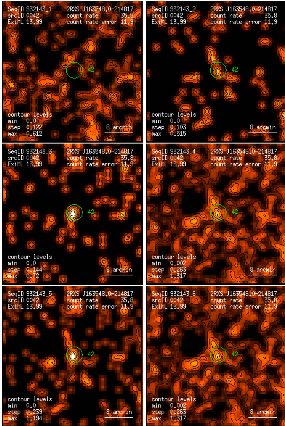
Figure 42: RASS 932143: detection 0042: band rate images, Gaussian filter: (1) PSPC channels 11 – 41, (2) 52 – 90, (3) 91 – 201, (4) 11 – 235, (5) 52 – 201, (6) 11 – 201. Broad band rates in counts/ks. Band rate contour levels in counts/ks/arcmin 2 .
