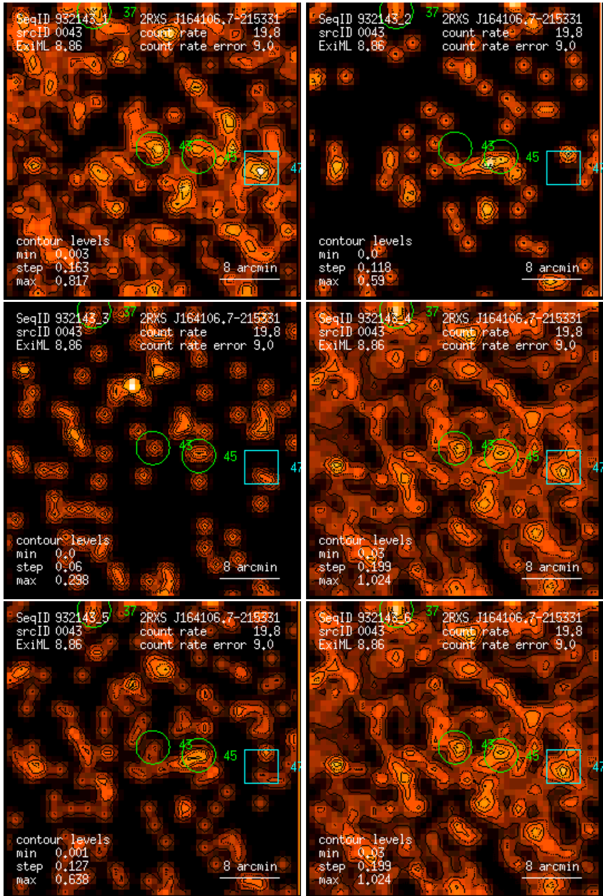
Figure 43: RASS 932143: detection 0043: band rate images, Gaussian filter: (1) PSPC channels 11 – 41, (2) 52 – 90, (3) 91 – 201, (4) 11 – 235, (5) 52 – 201, (6) 11 – 201. Broad band rates in counts/ks. Band rate contour levels in counts/ks/arcmin 2 .
