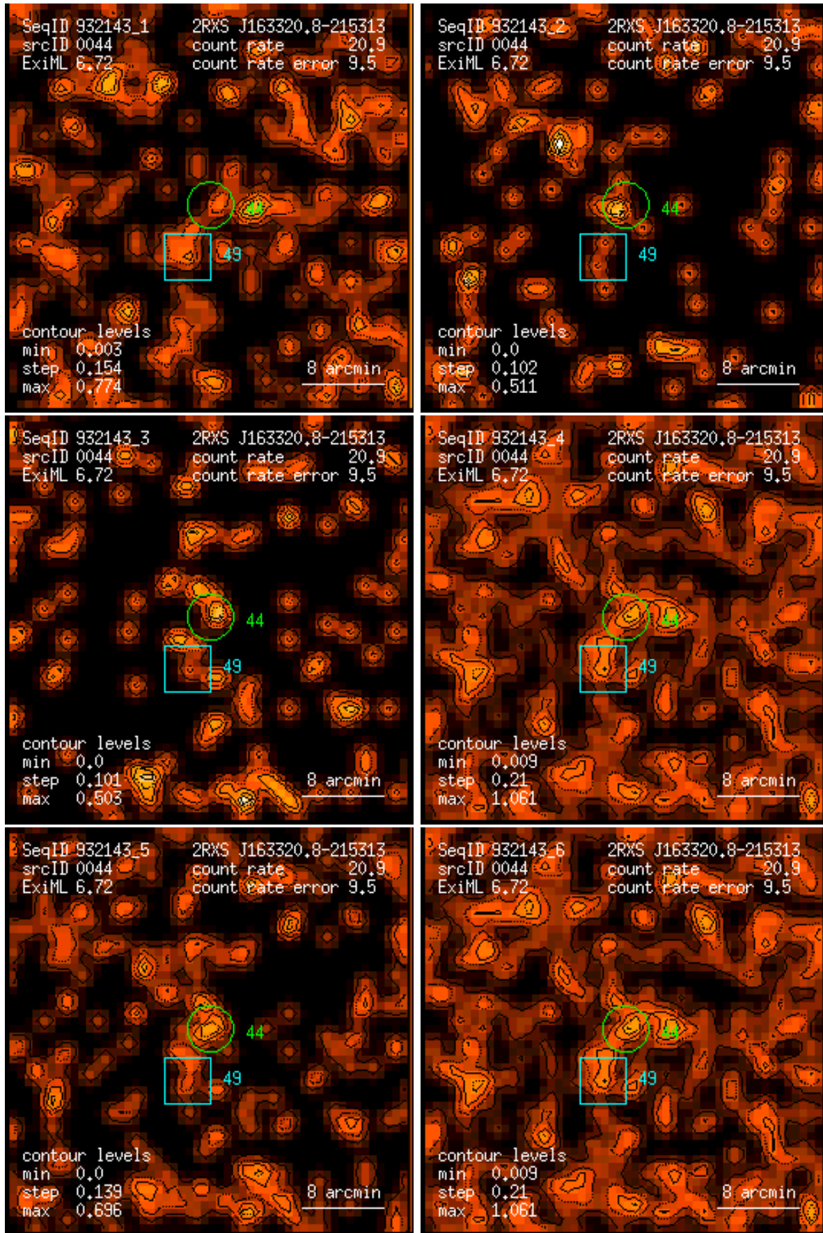
Figure 44: RASS 932143: detection 0044: band rate images, Gaussian filter: (1) PSPC channels 11 – 41, (2) 52 – 90, (3) 91 – 201, (4) 11 – 235, (5) 52 – 201, (6) 11 – 201. Broad band rates in counts/ks. Band rate contour levels in counts/ks/arcmin 2 .
