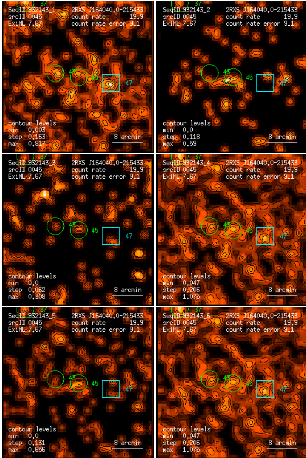
Figure 45: RASS 932143: detection 0045: band rate images, Gaussian filter: (1) PSPC channels 11 – 41, (2) 52 – 90, (3) 91 – 201, (4) 11 – 235, (5) 52 – 201, (6) 11 – 201. Broad band rates in counts/ks. Band rate contour levels in counts/ks/arcmin 2 .
