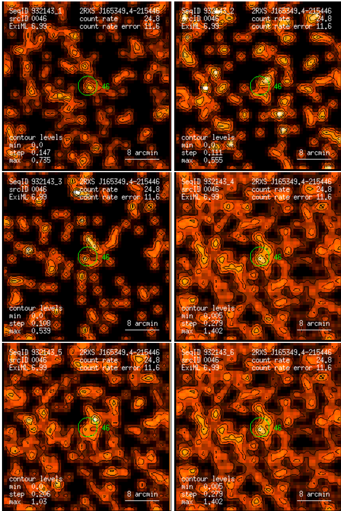
Figure 46: RASS 932143: detection 0046: band rate images, Gaussian filter: (1) PSPC channels 11 – 41, (2) 52 – 90, (3) 91 – 201, (4) 11 – 235, (5) 52 – 201, (6) 11 – 201. Broad band rates in counts/ks. Band rate contour levels in counts/ks/arcmin 2 .
