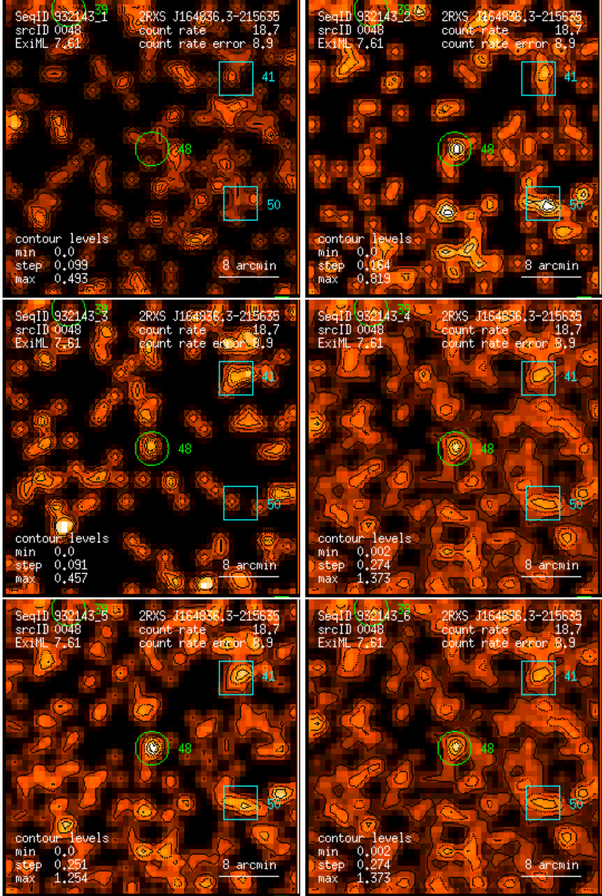
Figure 48: RASS 932143: detection 0048: band rate images, Gaussian filter: (1) PSPC channels 11 – 41, (2) 52 – 90, (3) 91 – 201, (4) 11 – 235, (5) 52 – 201, (6) 11 – 201. Broad band rates in counts/ks. Band rate contour levels in counts/ks/arcmin 2 .
