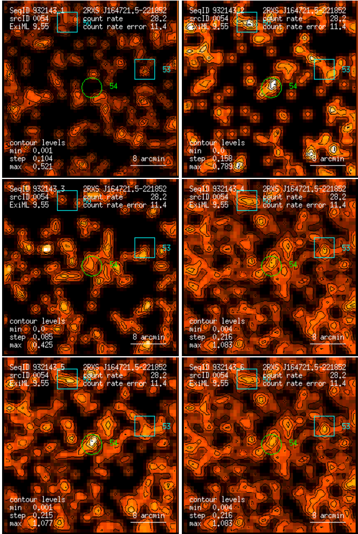
Figure 54: RASS 932143: detection 0054: band rate images, Gaussian filter: (1) PSPC channels 11 – 41, (2) 52 – 90, (3) 91 – 201, (4) 11 – 235, (5) 52 – 201, (6) 11 – 201. Broad band rates in counts/ks. Band rate contour levels in counts/ks/arcmin 2 .
