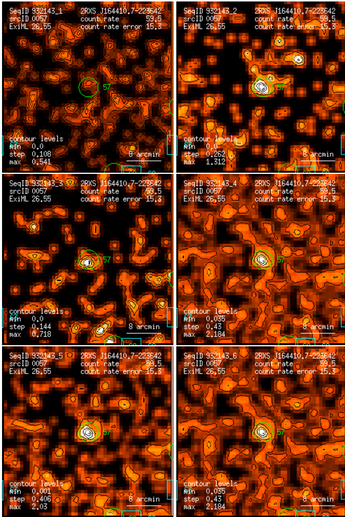
Figure 57: RASS 932143: detection 0057: band rate images, Gaussian filter: (1) PSPC channels 11 – 41, (2) 52 – 90, (3) 91 – 201, (4) 11 – 235, (5) 52 – 201, (6) 11 – 201. Broad band rates in counts/ks. Band rate contour levels in counts/ks/arcmin 2 .
