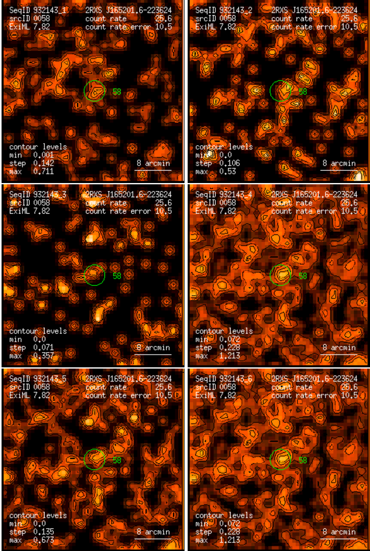
Figure 58: RASS 932143: detection 0058: band rate images, Gaussian filter: (1) PSPC channels 11 – 41, (2) 52 – 90, (3) 91 – 201, (4) 11 – 235, (5) 52 – 201, (6) 11 – 201. Broad band rates in counts/ks. Band rate contour levels in counts/ks/arcmin 2 .
