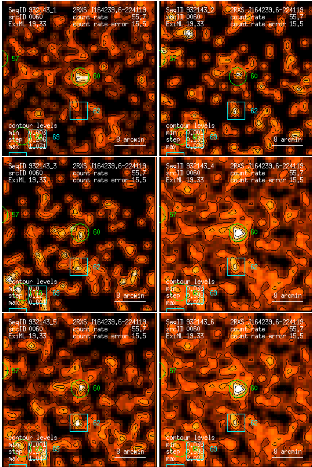
Figure 60: RASS 932143: detection 0060: band rate images, Gaussian filter: (1) PSPC channels 11 – 41, (2) 52 – 90, (3) 91 – 201, (4) 11 – 235, (5) 52 – 201, (6) 11 – 201. Broad band rates in counts/ks. Band rate contour levels in counts/ks/arcmin 2 .
