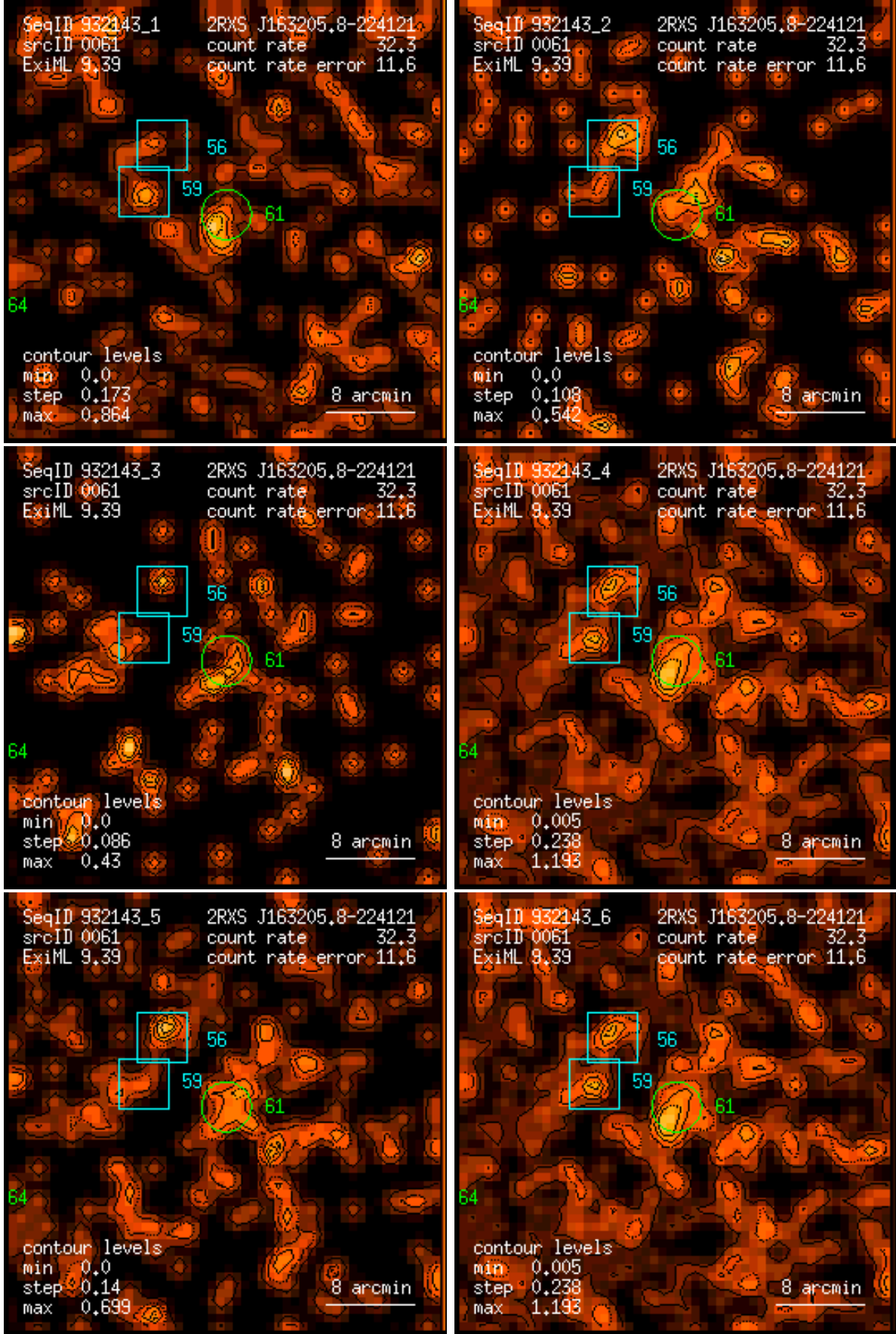
Figure 61: RASS 932143: detection 0061: band rate images, Gaussian filter: (1) PSPC channels 11 – 41, (2) 52 – 90, (3) 91 – 201, (4) 11 – 235, (5) 52 – 201, (6) 11 – 201. Broad band rates in counts/ks. Band rate contour levels in counts/ks/arcmin 2 .
