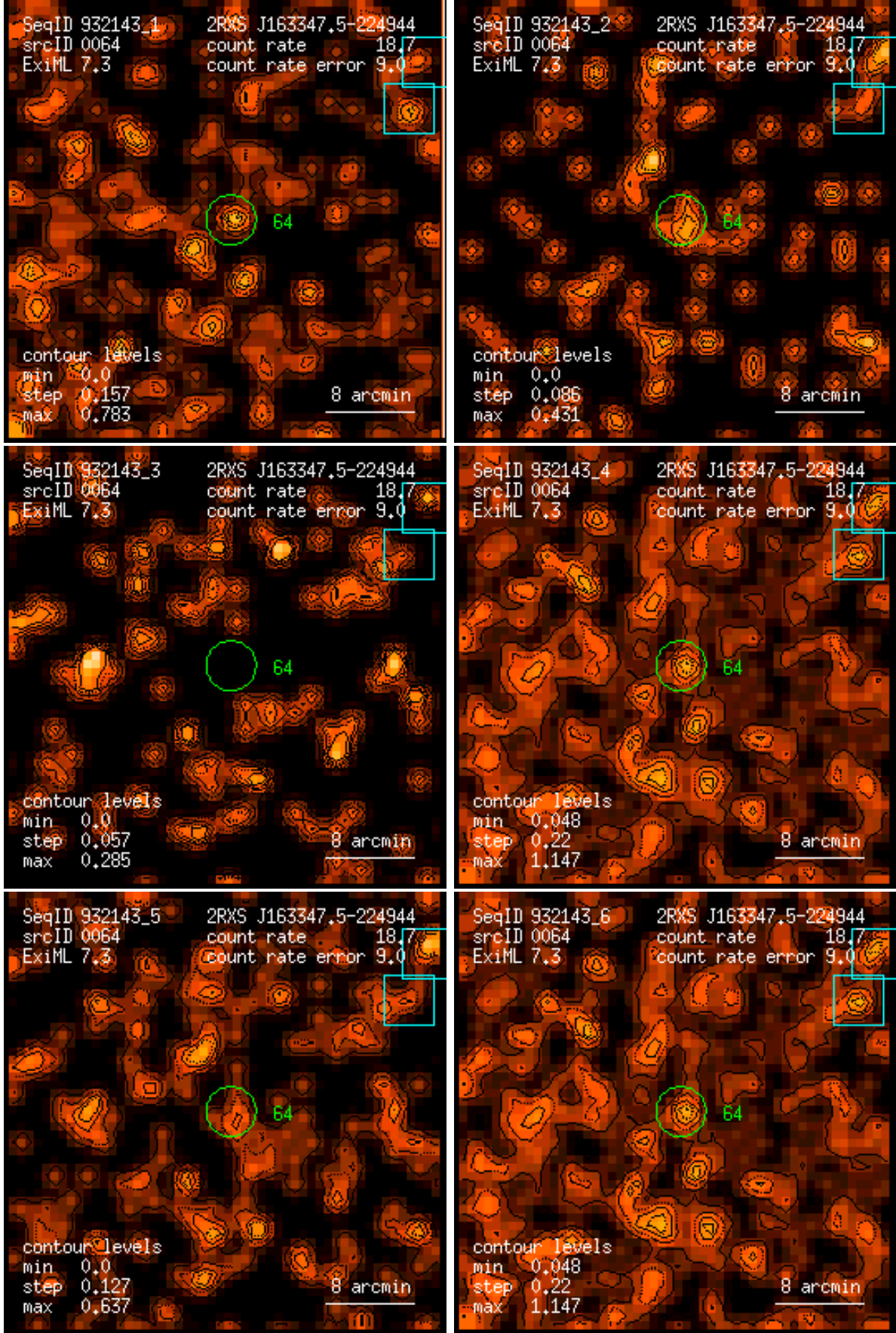
Figure 64: RASS 932143: detection 0064: band rate images, Gaussian filter: (1) PSPC channels 11 – 41, (2) 52 – 90, (3) 91 – 201, (4) 11 – 235, (5) 52 – 201, (6) 11 – 201. Broad band rates in counts/ks. Band rate contour levels in counts/ks/arcmin 2 .
