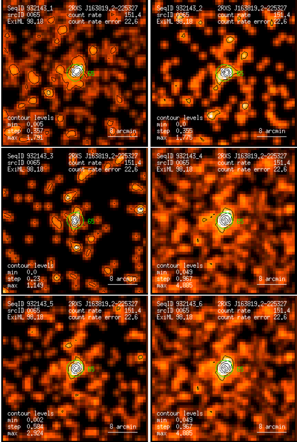
Figure 65: RASS 932143: detection 0065: band rate images, Gaussian filter: (1) PSPC channels 11 – 41, (2) 52 – 90, (3) 91 – 201, (4) 11 – 235, (5) 52 – 201, (6) 11 – 201. Broad band rates in counts/ks. Band rate contour levels in counts/ks/arcmin 2 .
