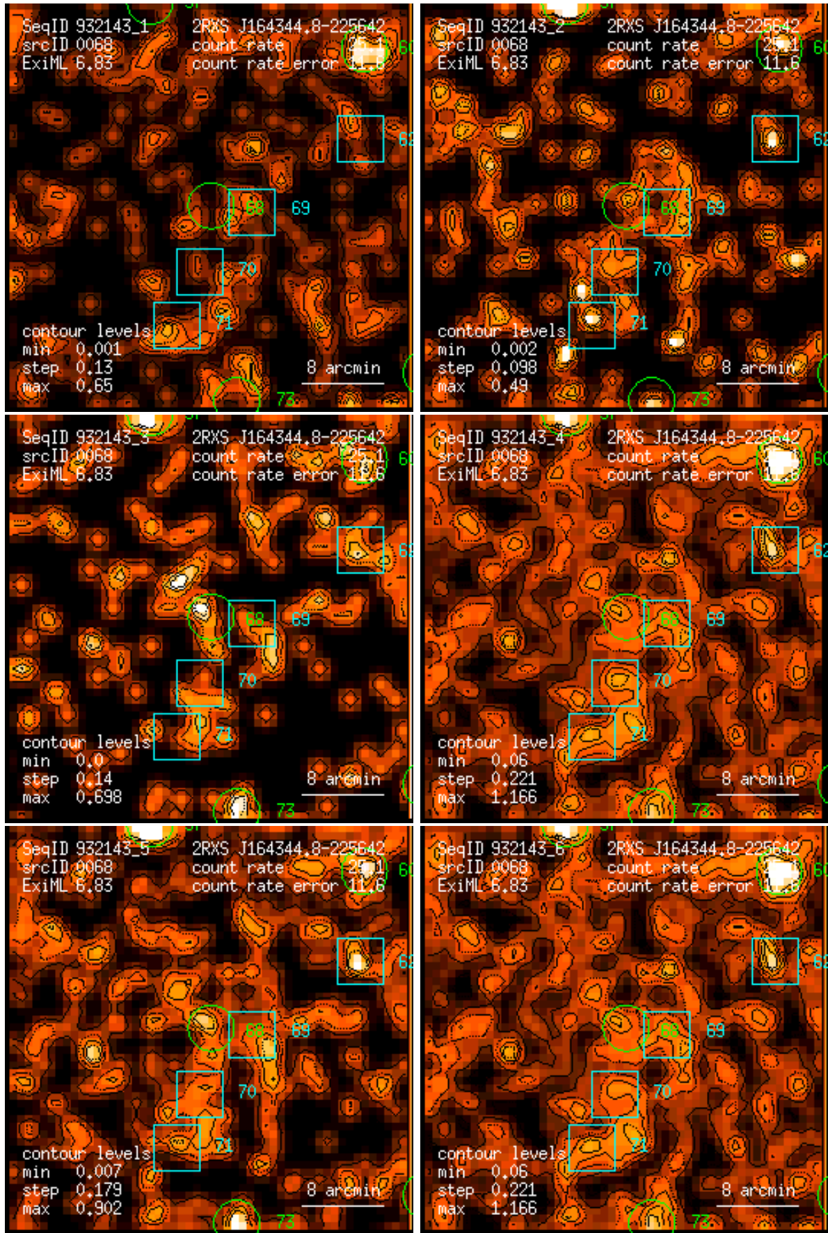
Figure 68: RASS 932143: detection 0068: band rate images, Gaussian filter: (1) PSPC channels 11 – 41, (2) 52 – 90, (3) 91 – 201, (4) 11 – 235, (5) 52 – 201, (6) 11 – 201. Broad band rates in counts/ks. Band rate contour levels in counts/ks/arcmin 2 .
