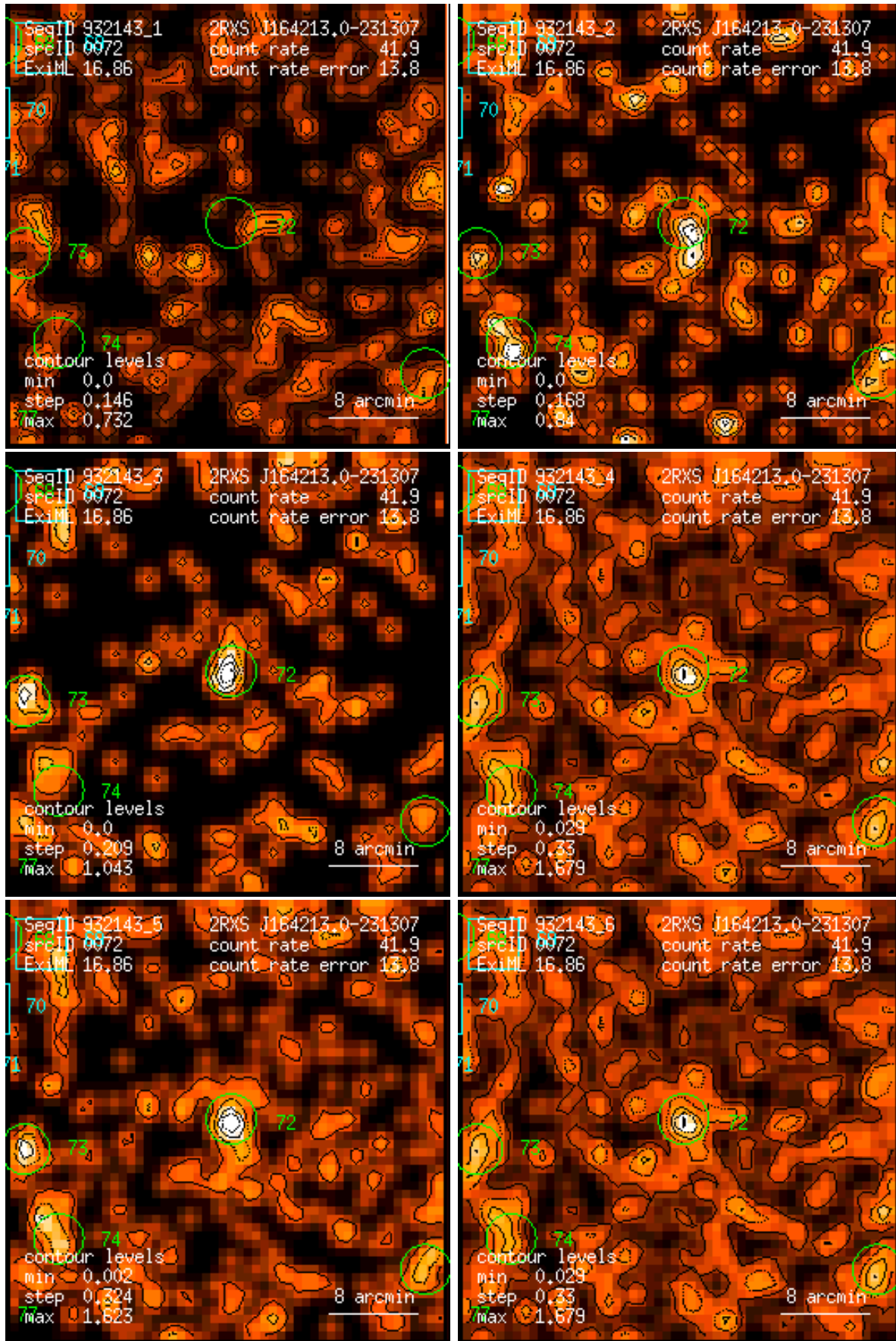
Figure 72: RASS 932143: detection 0072: band rate images, Gaussian filter: (1) PSPC channels 11 – 41, (2) 52 – 90, (3) 91 – 201, (4) 11 – 235, (5) 52 – 201, (6) 11 – 201. Broad band rates in counts/ks. Band rate contour levels in counts/ks/arcmin 2 .
