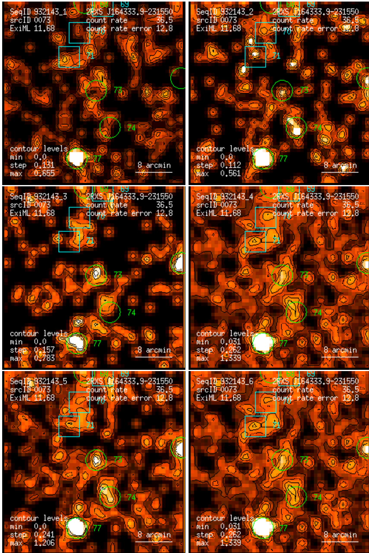
Figure 73: RASS 932143: detection 0073: band rate images, Gaussian filter: (1) PSPC channels 11 – 41, (2) 52 – 90, (3) 91 – 201, (4) 11 – 235, (5) 52 – 201, (6) 11 – 201. Broad band rates in counts/ks. Band rate contour levels in counts/ks/arcmin 2 .
