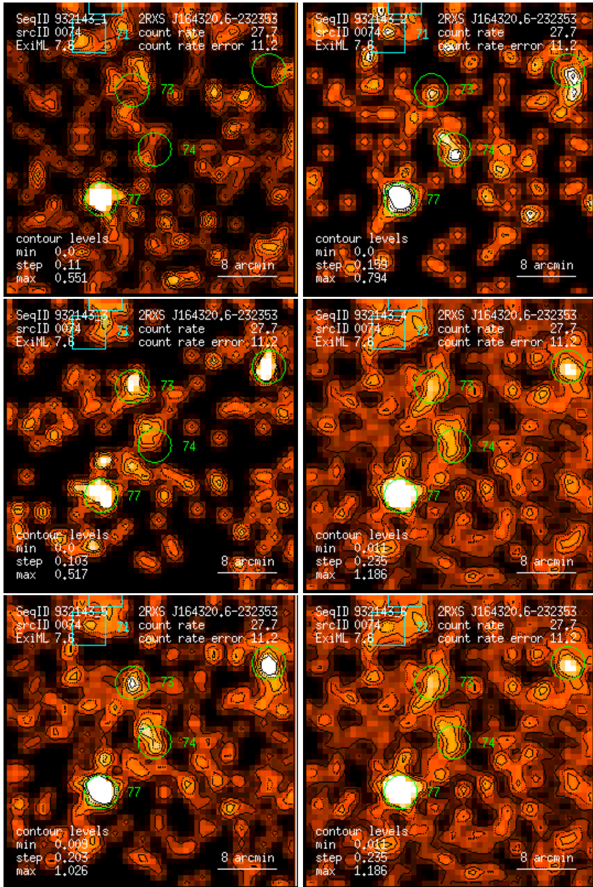
Figure 74: RASS 932143: detection 0074: band rate images, Gaussian filter: (1) PSPC channels 11 – 41, (2) 52 – 90, (3) 91 – 201, (4) 11 – 235, (5) 52 – 201, (6) 11 – 201. Broad band rates in counts/ks. Band rate contour levels in counts/ks/arcmin 2 .
