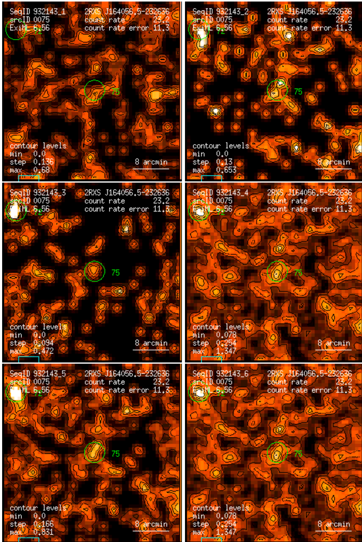
Figure 75: RASS 932143: detection 0075: band rate images, Gaussian filter: (1) PSPC channels 11 – 41, (2) 52 – 90, (3) 91 – 201, (4) 11 – 235, (5) 52 – 201, (6) 11 – 201. Broad band rates in counts/ks. Band rate contour levels in counts/ks/arcmin 2 .
