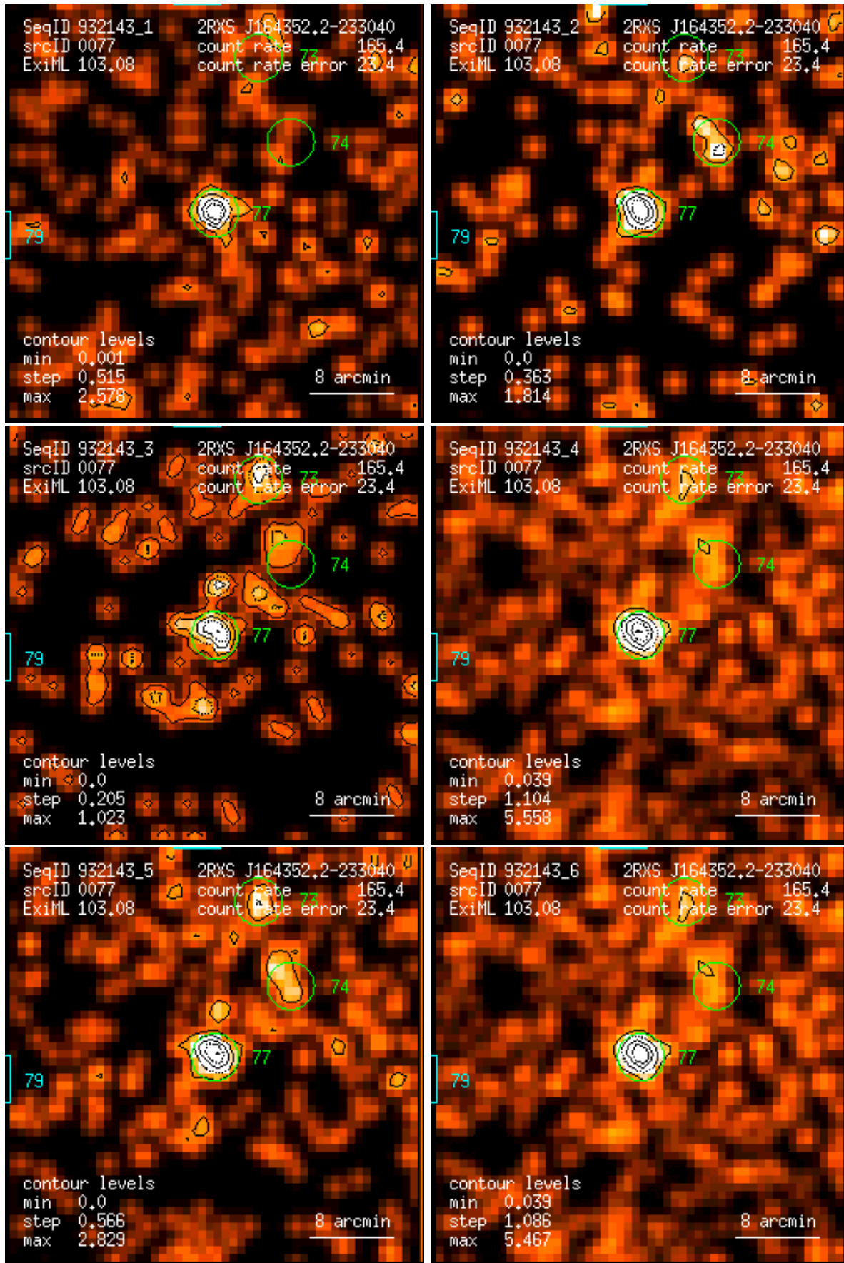
Figure 77: RASS 932143: detection 0077: band rate images, Gaussian filter: (1) PSPC channels 11 – 41, (2) 52 – 90, (3) 91 – 201, (4) 11 – 235, (5) 52 – 201, (6) 11 – 201. Broad band rates in counts/ks. Band rate contour levels in counts/ks/arcmin 2 .
