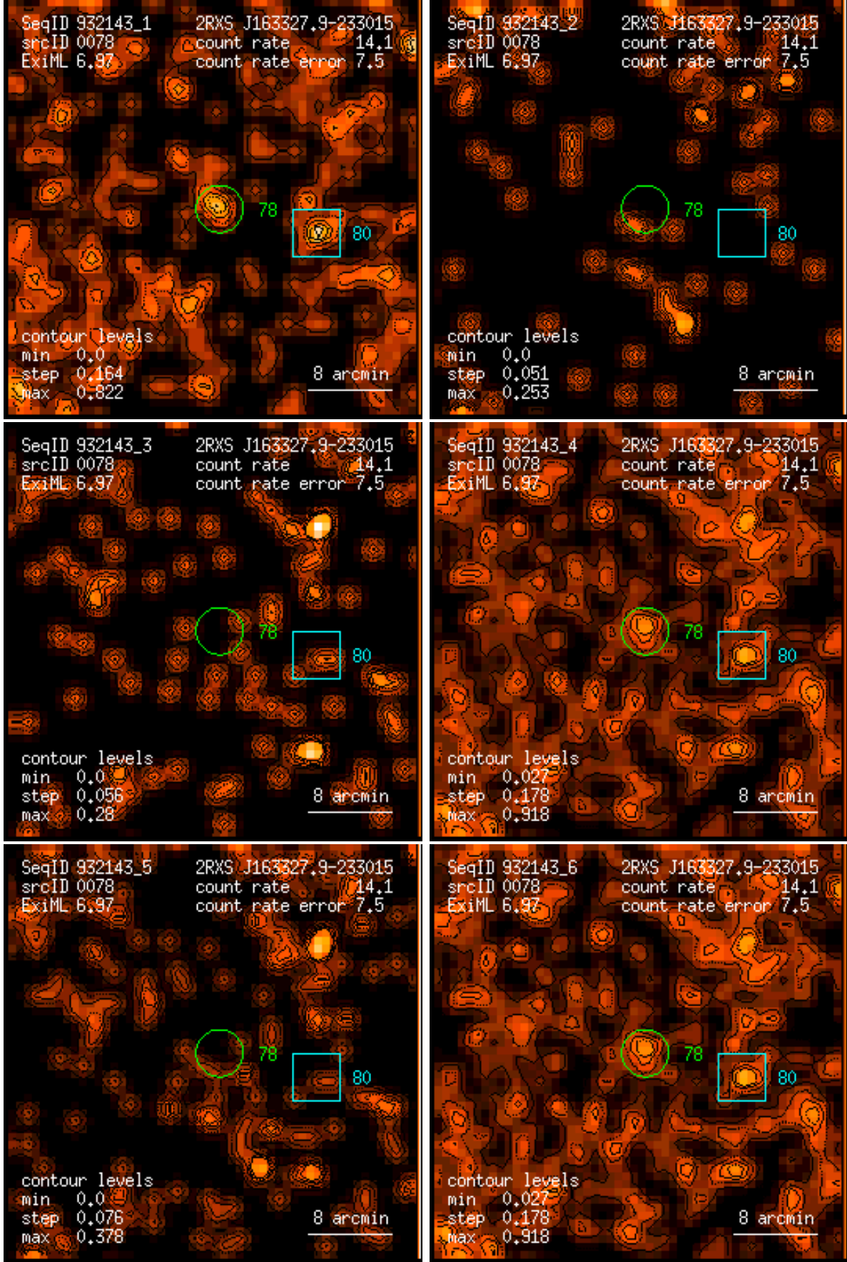
Figure 78: RASS 932143: detection 0078: band rate images, Gaussian filter: (1) PSPC channels 11 – 41, (2) 52 – 90, (3) 91 – 201, (4) 11 – 235, (5) 52 – 201, (6) 11 – 201. Broad band rates in counts/ks. Band rate contour levels in counts/ks/arcmin 2 .
