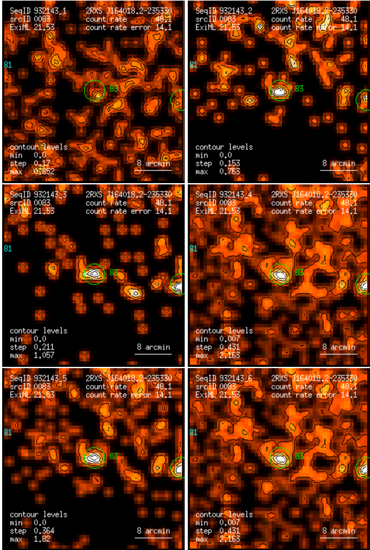
Figure 83: RASS 932143: detection 0083: band rate images, Gaussian filter: (1) PSPC channels 11 – 41, (2) 52 – 90, (3) 91 – 201, (4) 11 – 235, (5) 52 – 201, (6) 11 – 201. Broad band rates in counts/ks. Band rate contour levels in counts/ks/arcmin 2 .
