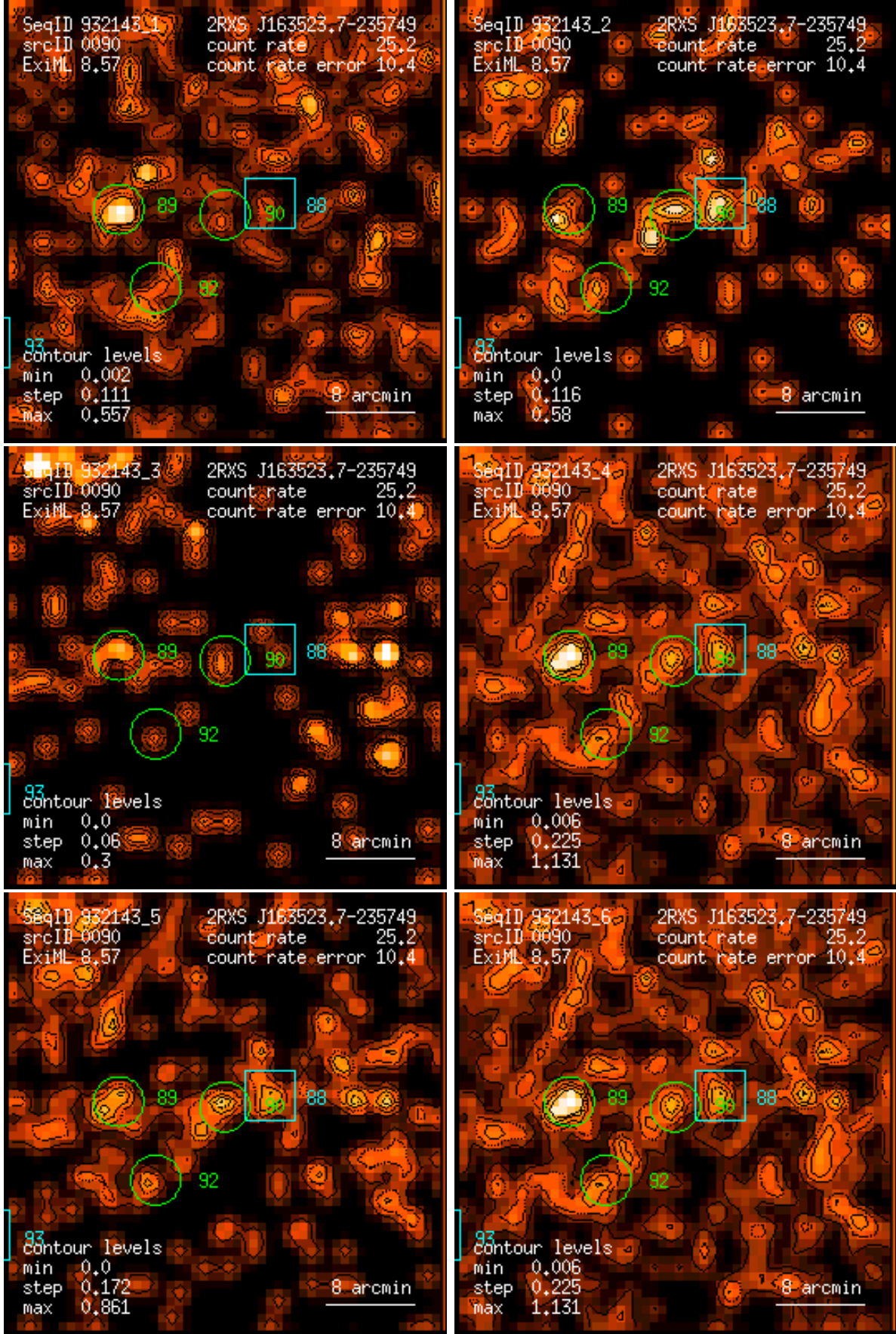
Figure 90: RASS 932143: detection 0090: band rate images, Gaussian filter: (1) PSPC channels 11 – 41, (2) 52 – 90, (3) 91 – 201, (4) 11 – 235, (5) 52 – 201, (6) 11 – 201. Broad band rates in counts/ks. Band rate contour levels in counts/ks/arcmin 2 .
