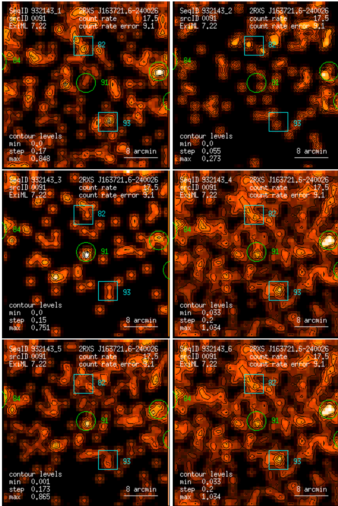
Figure 91: RASS 932143: detection 0091: band rate images, Gaussian filter: (1) PSPC channels 11 – 41, (2) 52 – 90, (3) 91 – 201, (4) 11 – 235, (5) 52 – 201, (6) 11 – 201. Broad band rates in counts/ks. Band rate contour levels in counts/ks/arcmin 2 .
