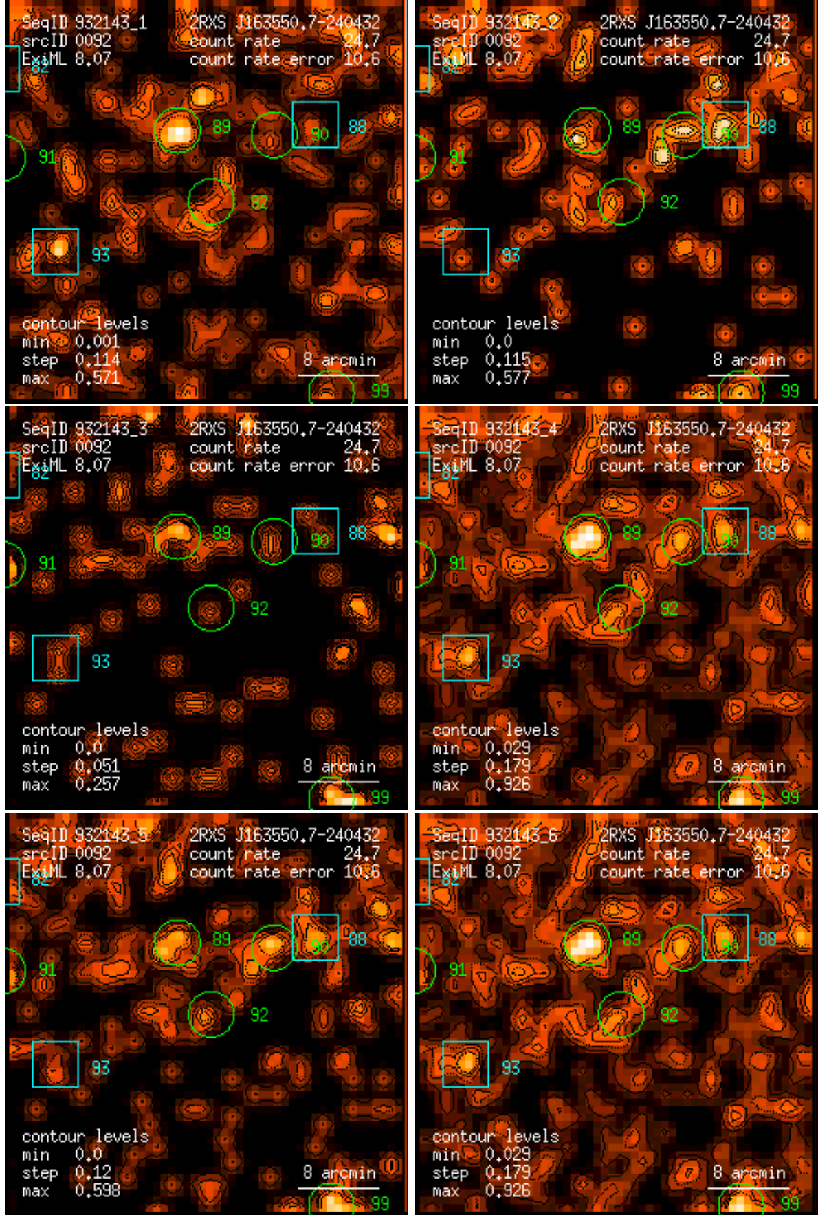
Figure 92: RASS 932143: detection 0092: band rate images, Gaussian filter: (1) PSPC channels 11 – 41, (2) 52 – 90, (3) 91 – 201, (4) 11 – 235, (5) 52 – 201, (6) 11 – 201. Broad band rates in counts/ks. Band rate contour levels in counts/ks/arcmin 2 .
