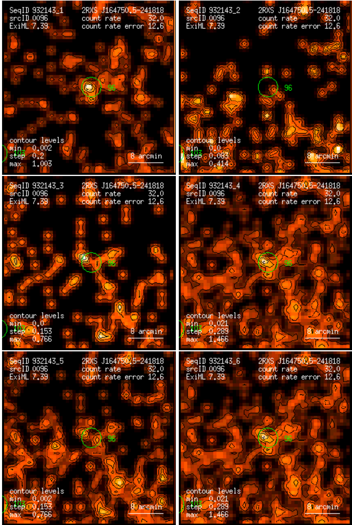
Figure 96: RASS 932143: detection 0096: band rate images, Gaussian filter: (1) PSPC channels 11 – 41, (2) 52 – 90, (3) 91 – 201, (4) 11 – 235, (5) 52 – 201, (6) 11 – 201. Broad band rates in counts/ks. Band rate contour levels in counts/ks/arcmin 2 .
