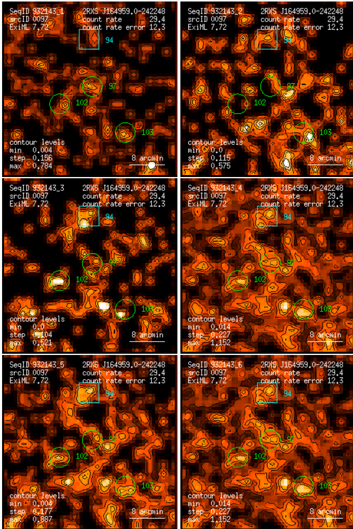
Figure 97: RASS 932143: detection 0097: band rate images, Gaussian filter: (1) PSPC channels 11 – 41, (2) 52 – 90, (3) 91 – 201, (4) 11 – 235, (5) 52 – 201, (6) 11 – 201. Broad band rates in counts/ks. Band rate contour levels in counts/ks/arcmin 2 .
