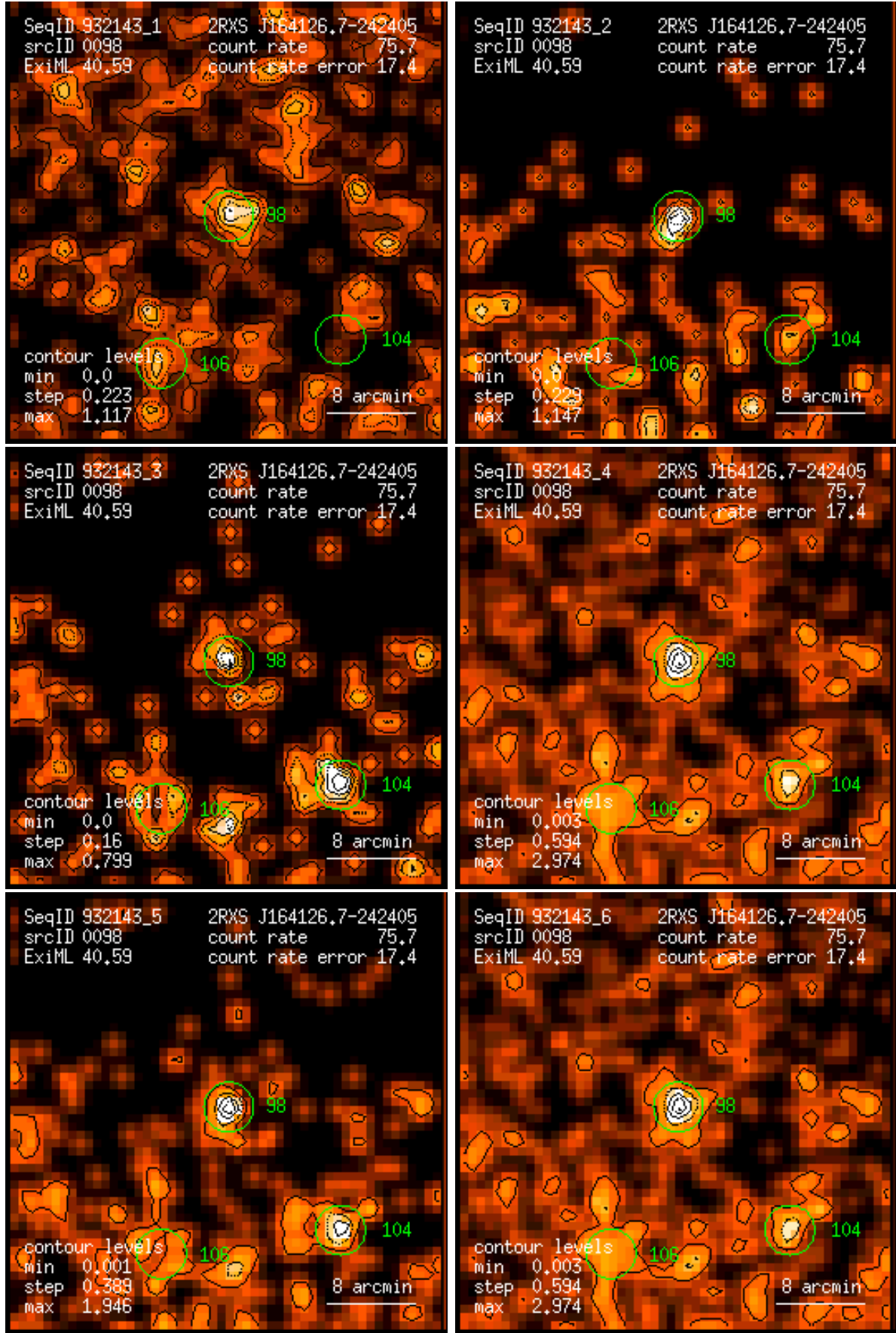
Figure 98: RASS 932143: detection 0098: band rate images, Gaussian filter: (1) PSPC channels 11 – 41, (2) 52 – 90, (3) 91 – 201, (4) 11 – 235, (5) 52 – 201, (6) 11 – 201. Broad band rates in counts/ks. Band rate contour levels in counts/ks/arcmin 2 .
