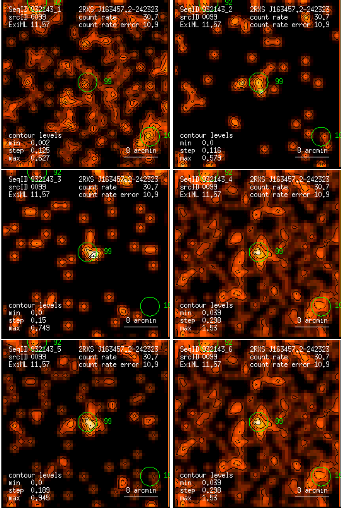
Figure 99: RASS 932143: detection 0099: band rate images, Gaussian filter: (1) PSPC channels 11 – 41, (2) 52 – 90, (3) 91 – 201, (4) 11 – 235, (5) 52 – 201, (6) 11 – 201. Broad band rates in counts/ks. Band rate contour levels in counts/ks/arcmin 2 .
