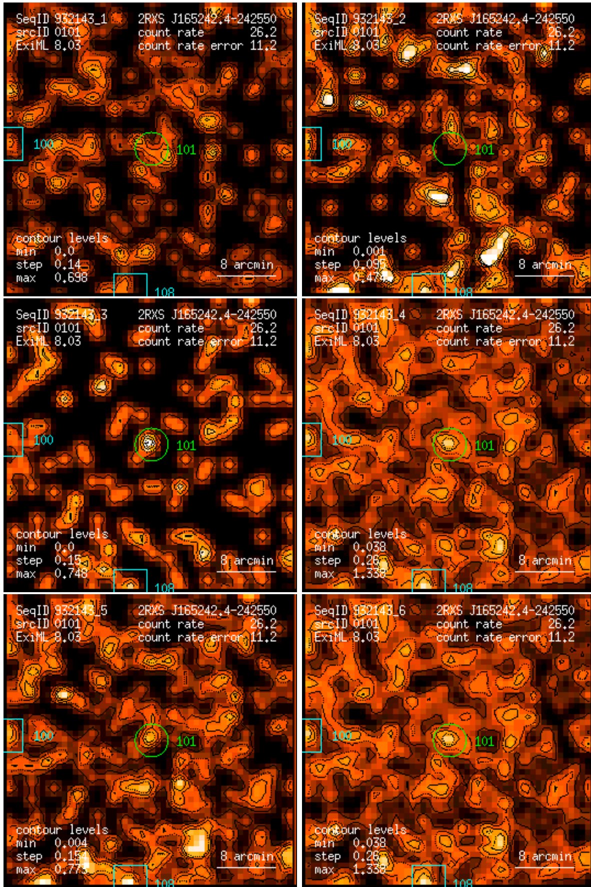
Figure 101: RASS 932143: detection 0101: band rate images, Gaussian filter: (1) PSPC channels 11 – 41, (2) 52 – 90, (3) 91 – 201, (4) 11 – 235, (5) 52 – 201, (6) 11 – 201. Broad band rates in counts/ks. Band rate contour levels in counts/ks/arcmin 2 .
