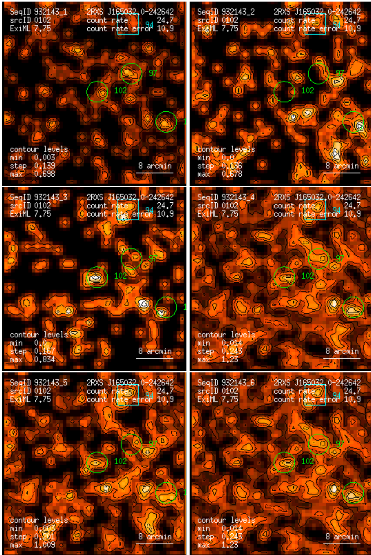
Figure 102: RASS 932143: detection 0102: band rate images, Gaussian filter: (1) PSPC channels 11 – 41, (2) 52 – 90, (3) 91 – 201, (4) 11 – 235, (5) 52 – 201, (6) 11 – 201. Broad band rates in counts/ks. Band rate contour levels in counts/ks/arcmin 2 .
