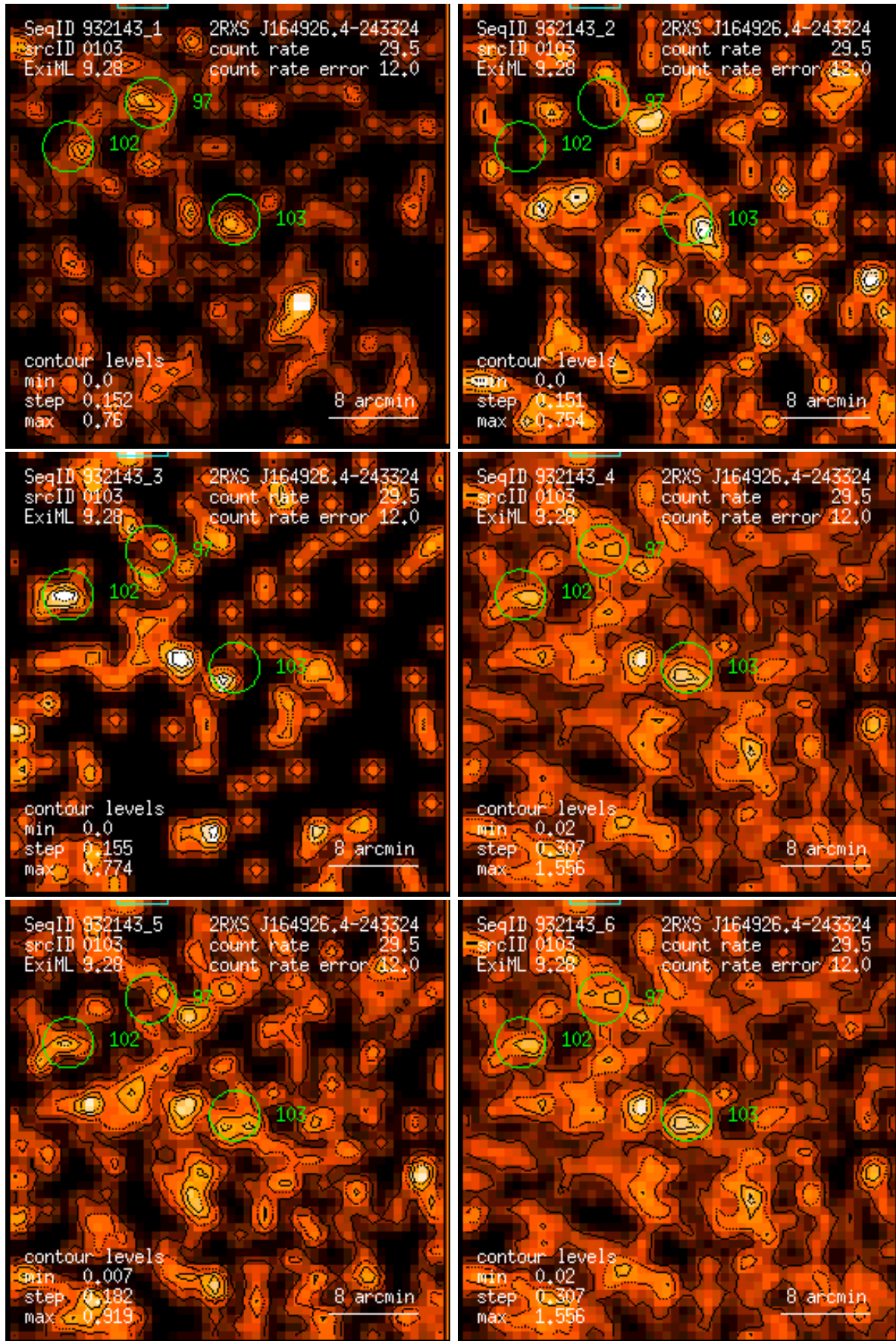
Figure 103: RASS 932143: detection 0103: band rate images, Gaussian filter: (1) PSPC channels 11 – 41, (2) 52 – 90, (3) 91 – 201, (4) 11 – 235, (5) 52 – 201, (6) 11 – 201. Broad band rates in counts/ks. Band rate contour levels in counts/ks/arcmin 2 .
