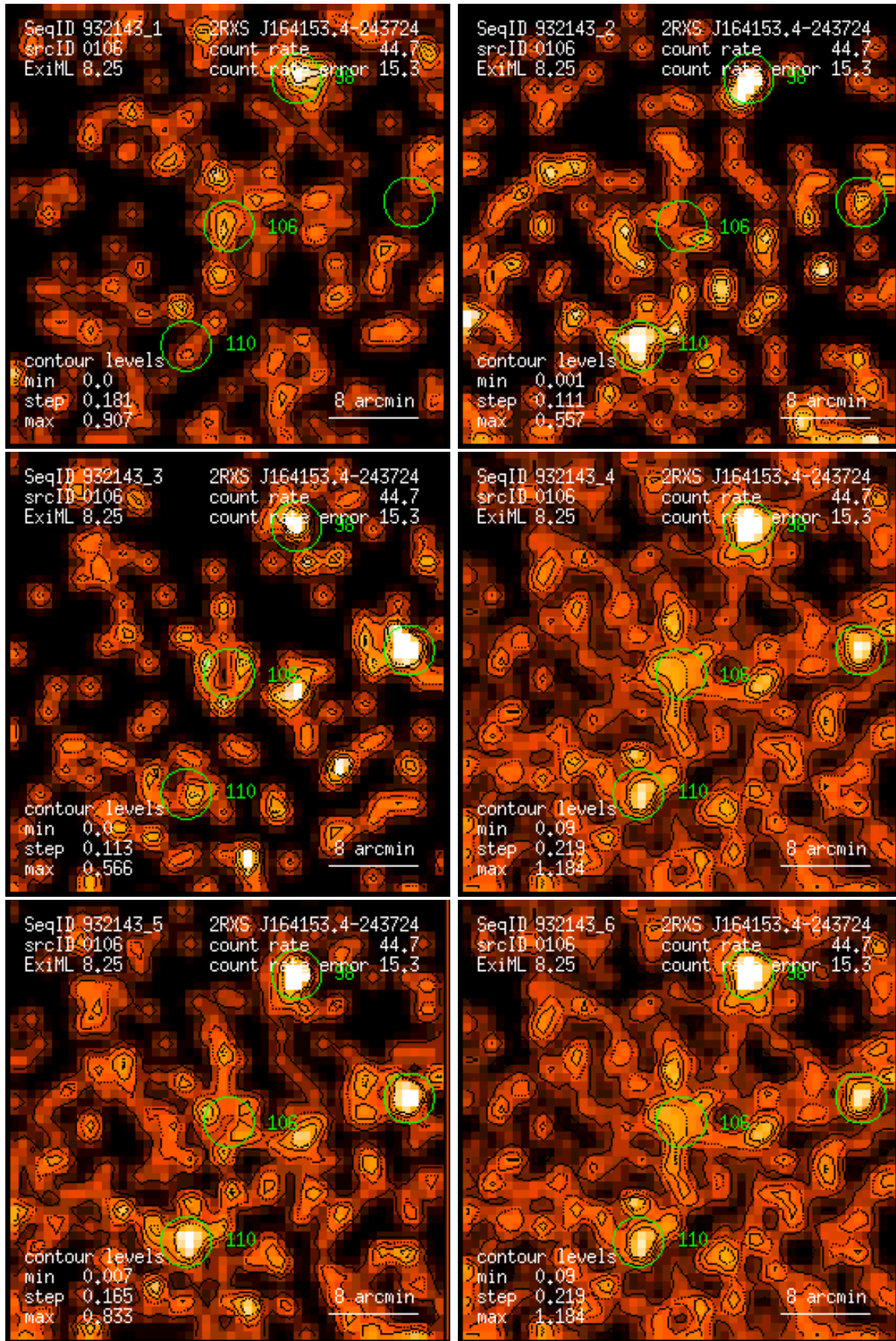
Figure 106: RASS 932143: detection 0106: band rate images, Gaussian filter: (1) PSPC channels 11 – 41, (2) 52 – 90, (3) 91 – 201, (4) 11 – 235, (5) 52 – 201, (6) 11 – 201. Broad band rates in counts/ks. Band rate contour levels in counts/ks/arcmin 2 .
