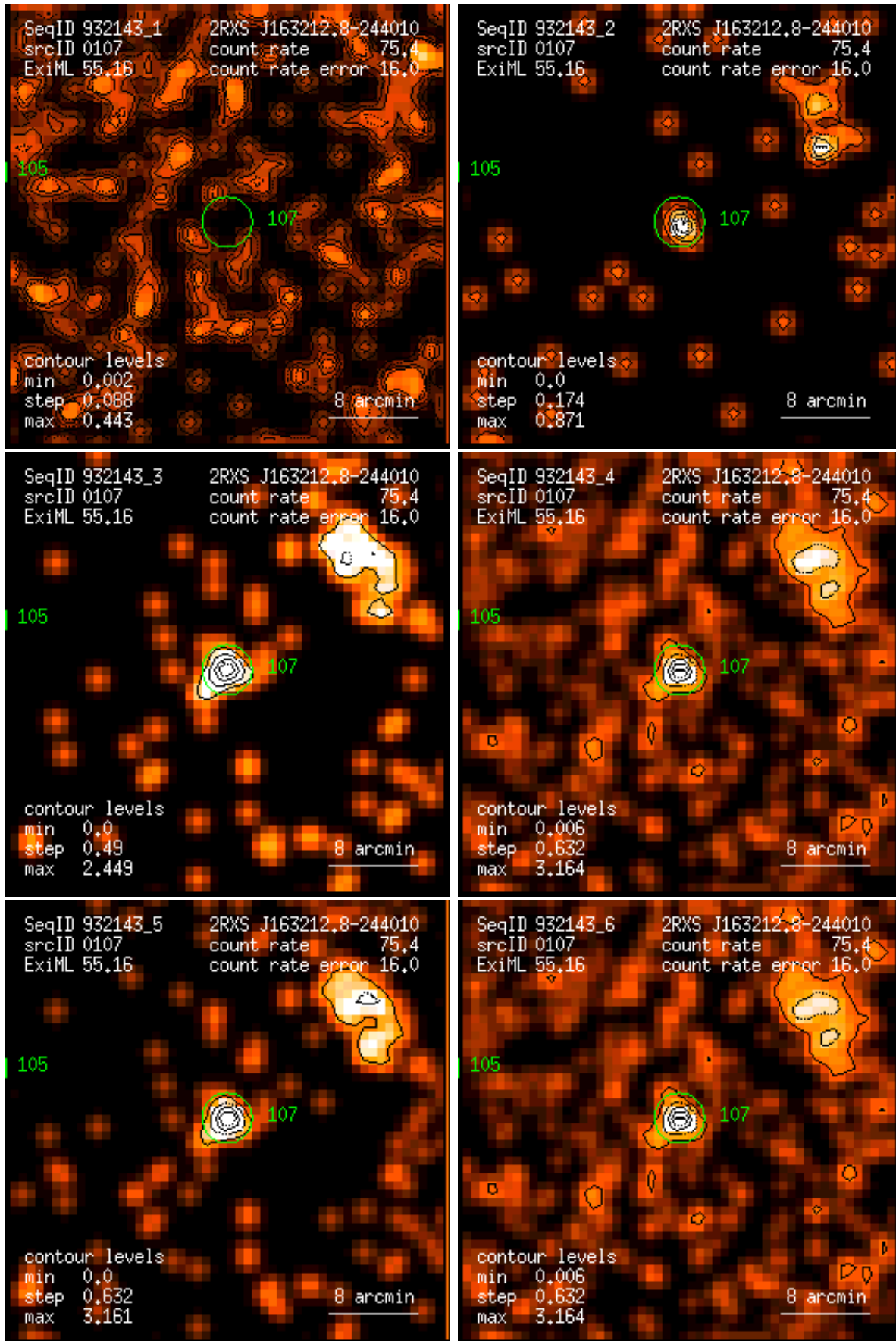
Figure 107: RASS 932143: detection 0107: band rate images, Gaussian filter: (1) PSPC channels 11 – 41, (2) 52 – 90, (3) 91 – 201, (4) 11 – 235, (5) 52 – 201, (6) 11 – 201. Broad band rates in counts/ks. Band rate contour levels in counts/ks/arcmin 2 .
