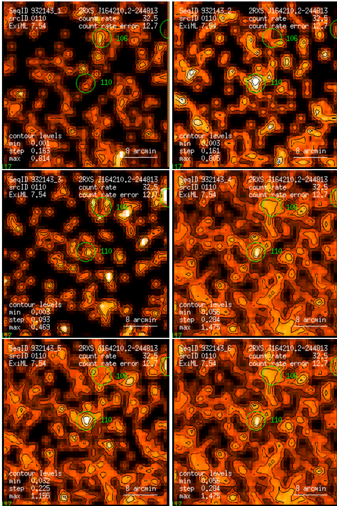
Figure 110: RASS 932143: detection 0110: band rate images, Gaussian filter: (1) PSPC channels 11 – 41, (2) 52 – 90, (3) 91 – 201, (4) 11 – 235, (5) 52 – 201, (6) 11 – 201. Broad band rates in counts/ks. Band rate contour levels in counts/ks/arcmin 2 .
