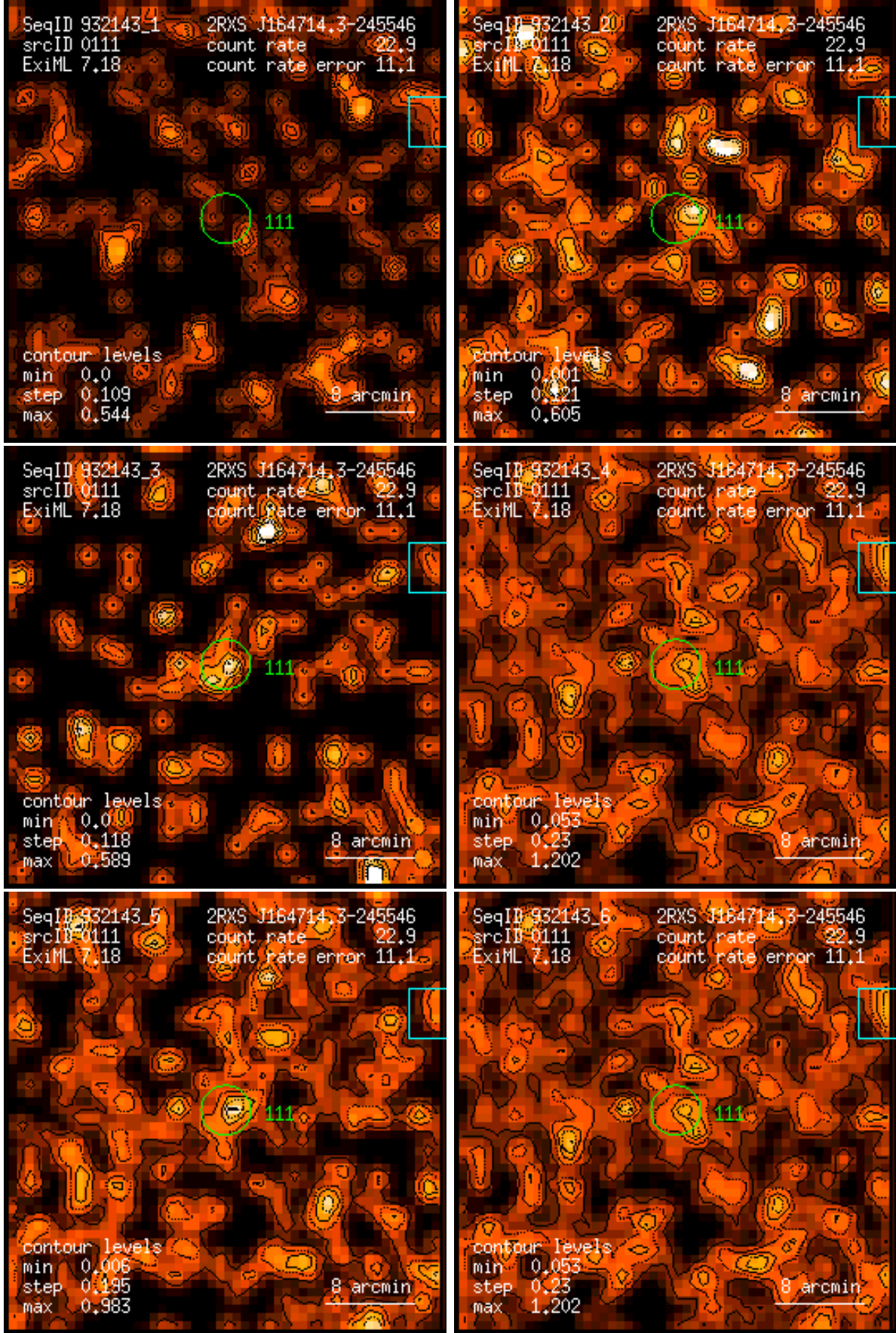
Figure 111: RASS 932143: detection 0111: band rate images, Gaussian filter: (1) PSPC channels 11 – 41, (2) 52 – 90, (3) 91 – 201, (4) 11 – 235, (5) 52 – 201, (6) 11 – 201. Broad band rates in counts/ks. Band rate contour levels in counts/ks/arcmin 2 .
