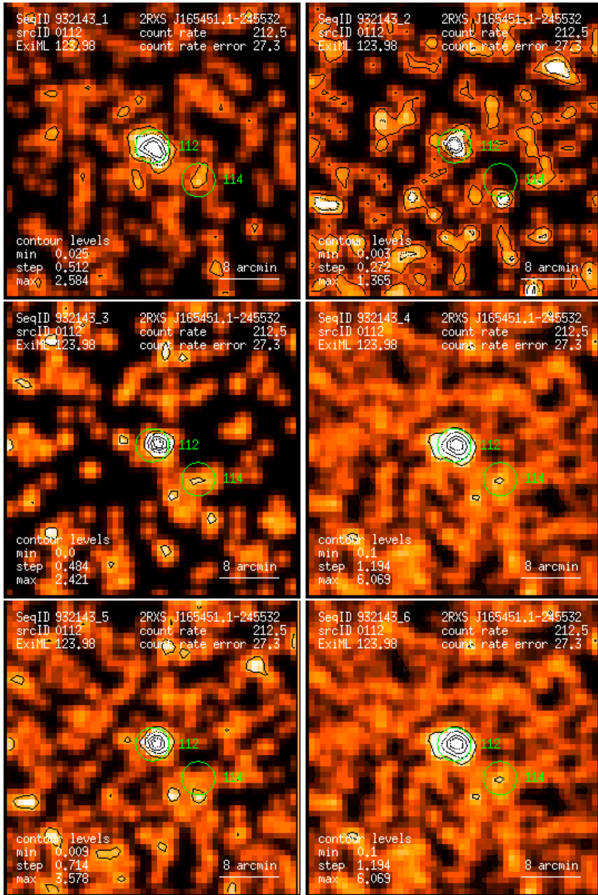
Figure 112: RASS 932143: detection 0112: band rate images, Gaussian filter: (1) PSPC channels 11 – 41, (2) 52 – 90, (3) 91 – 201, (4) 11 – 235, (5) 52 – 201, (6) 11 – 201. Broad band rates in counts/ks. Band rate contour levels in counts/ks/arcmin 2 .
