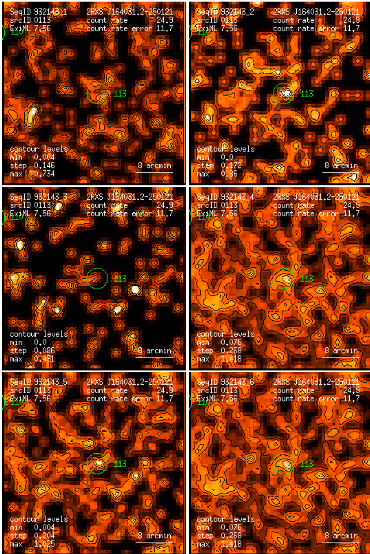
Figure 113: RASS 932143: detection 0113: band rate images, Gaussian filter: (1) PSPC channels 11 – 41, (2) 52 – 90, (3) 91 – 201, (4) 11 – 235, (5) 52 – 201, (6) 11 – 201. Broad band rates in counts/ks. Band rate contour levels in counts/ks/arcmin 2 .
