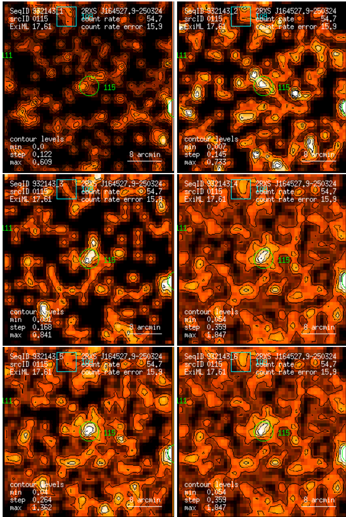
Figure 115: RASS 932143: detection 0115: band rate images, Gaussian filter: (1) PSPC channels 11 – 41, (2) 52 – 90, (3) 91 – 201, (4) 11 – 235, (5) 52 – 201, (6) 11 – 201. Broad band rates in counts/ks. Band rate contour levels in counts/ks/arcmin 2 .
