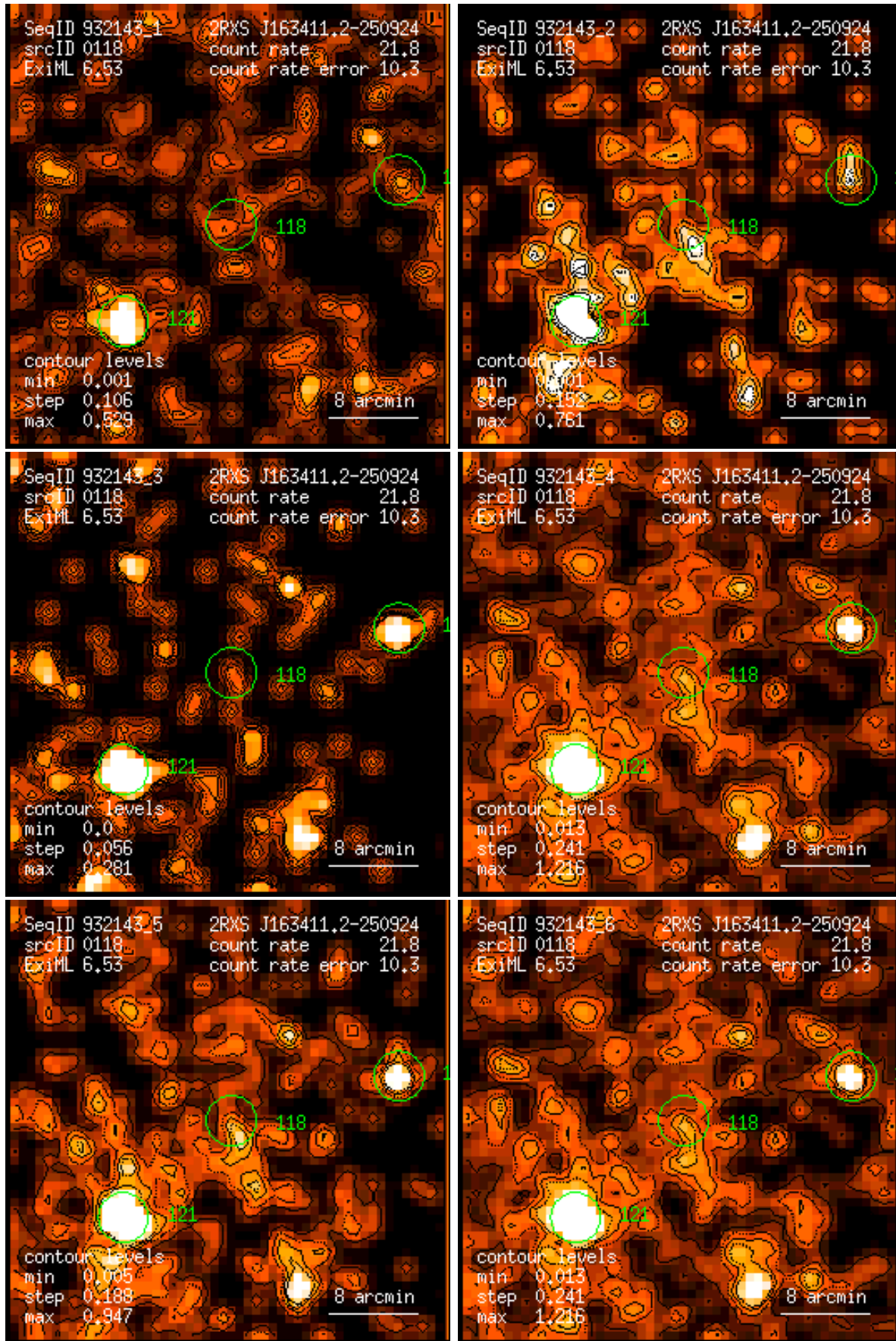
Figure 118: RASS 932143: detection 0118: band rate images, Gaussian filter: (1) PSPC channels 11 – 41, (2) 52 – 90, (3) 91 – 201, (4) 11 – 235, (5) 52 – 201, (6) 11 – 201. Broad band rates in counts/ks. Band rate contour levels in counts/ks/arcmin 2 .
