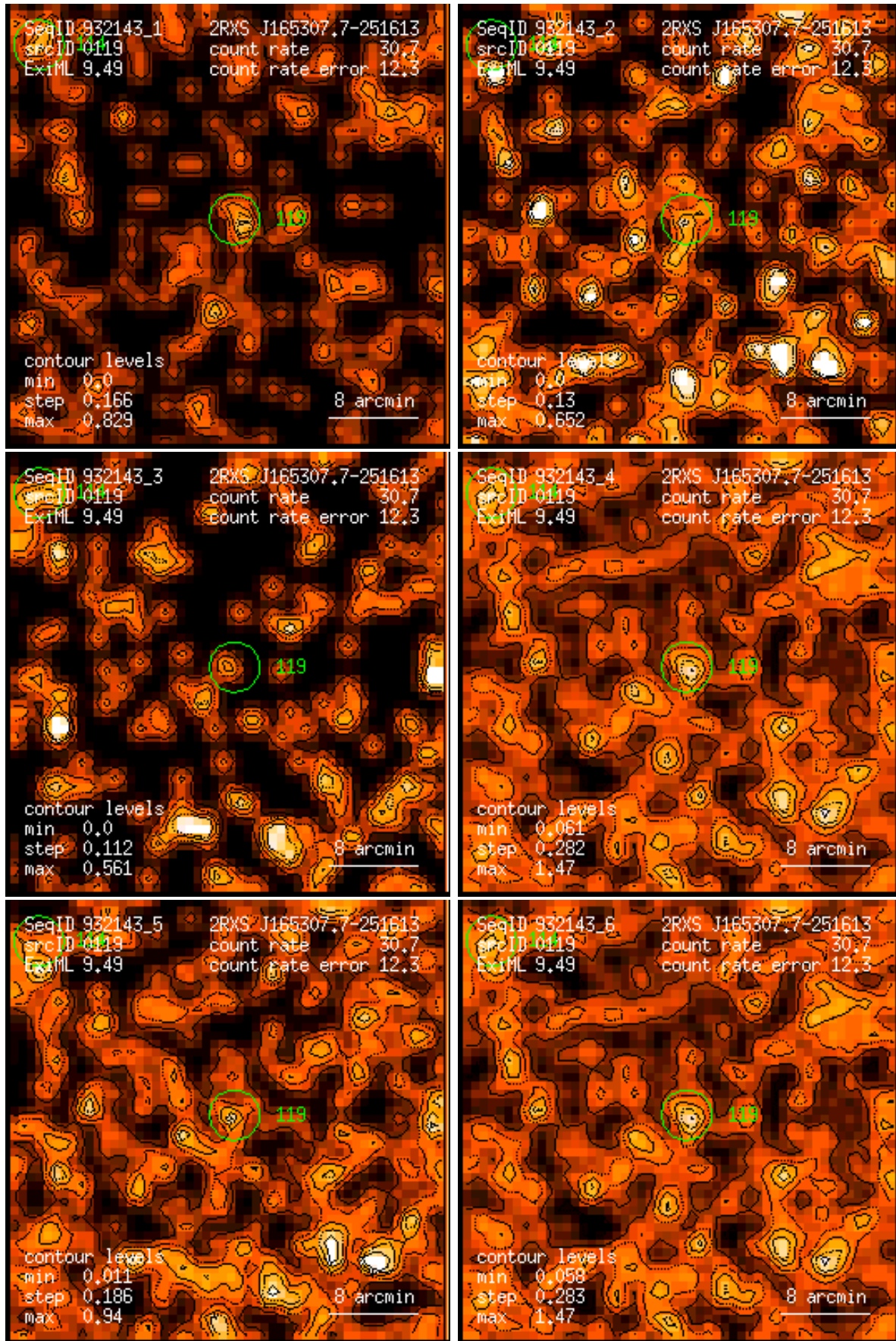
Figure 119: RASS 932143: detection 0119: band rate images, Gaussian filter: (1) PSPC channels 11 – 41, (2) 52 – 90, (3) 91 – 201, (4) 11 – 235, (5) 52 – 201, (6) 11 – 201. Broad band rates in counts/ks. Band rate contour levels in counts/ks/arcmin 2 .
