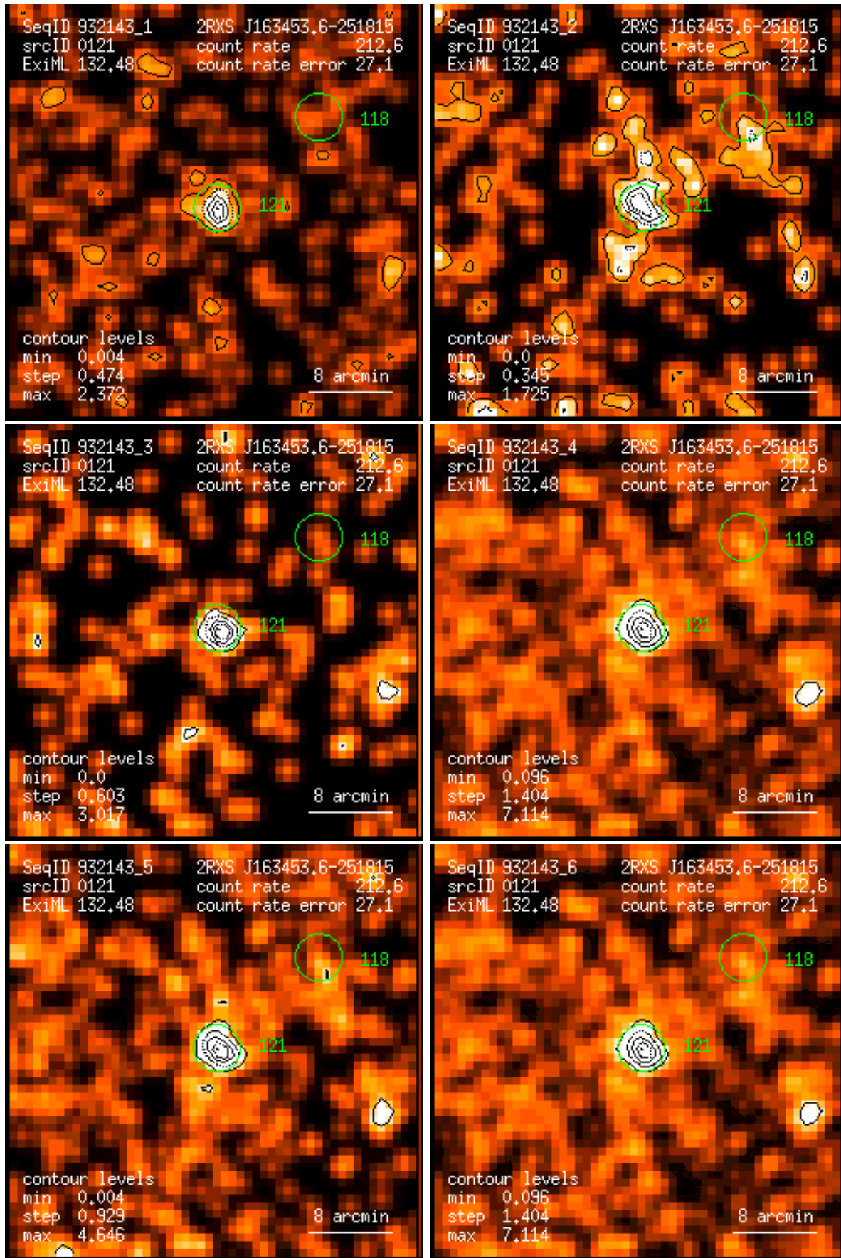
Figure 121: RASS 932143: detection 0121: band rate images, Gaussian filter: (1) PSPC channels 11 – 41, (2) 52 – 90, (3) 91 – 201, (4) 11 – 235, (5) 52 – 201, (6) 11 – 201. Broad band rates in counts/ks. Band rate contour levels in counts/ks/arcmin 2 .
