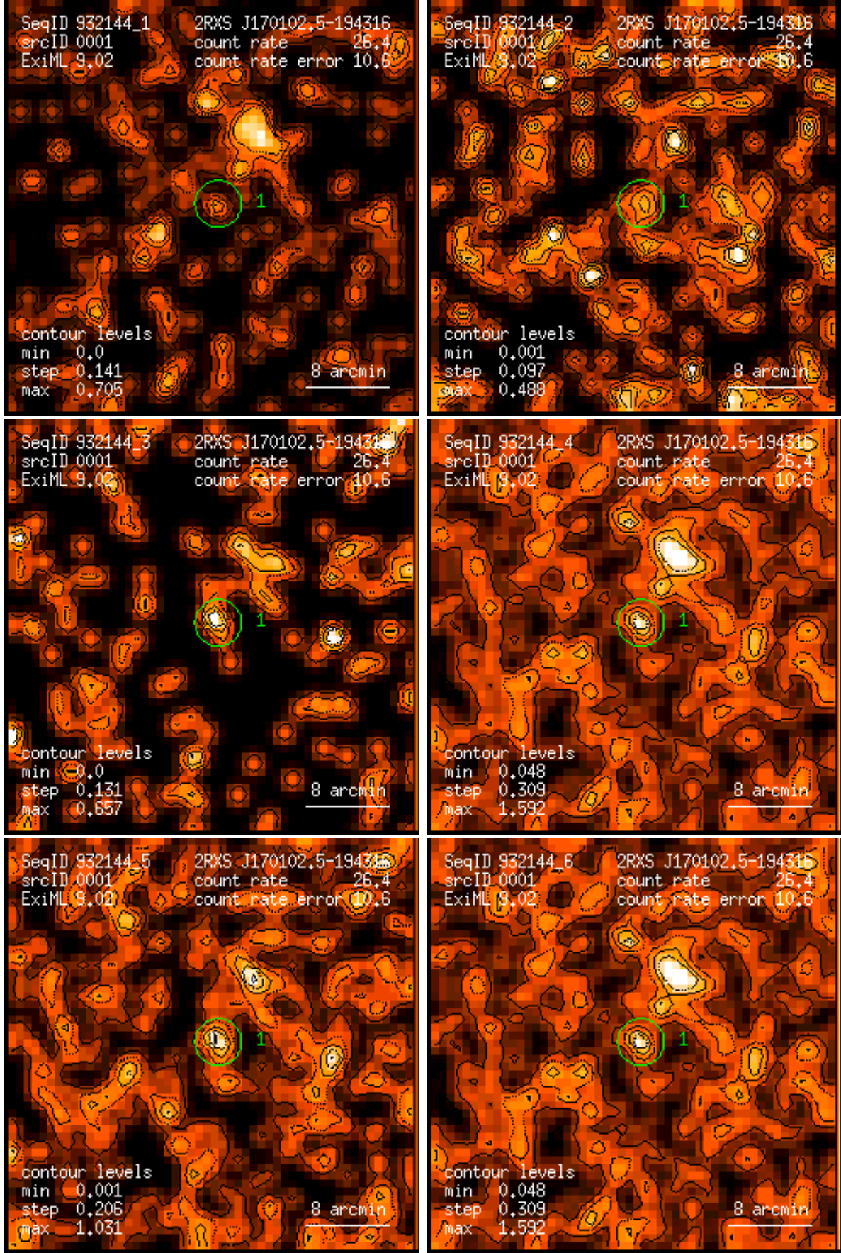
Figure 1: RASS 932144: detection 0001: band rate images, Gaussian filter: (1) PSPC channels 11 – 41, (2) 52 – 90, (3) 91 – 201, (4) 11 – 235, (5) 52 – 201, (6) 11 – 201. Broad band rates in counts/ks. Band rate contour levels in counts/ks/arcmin 2 .
