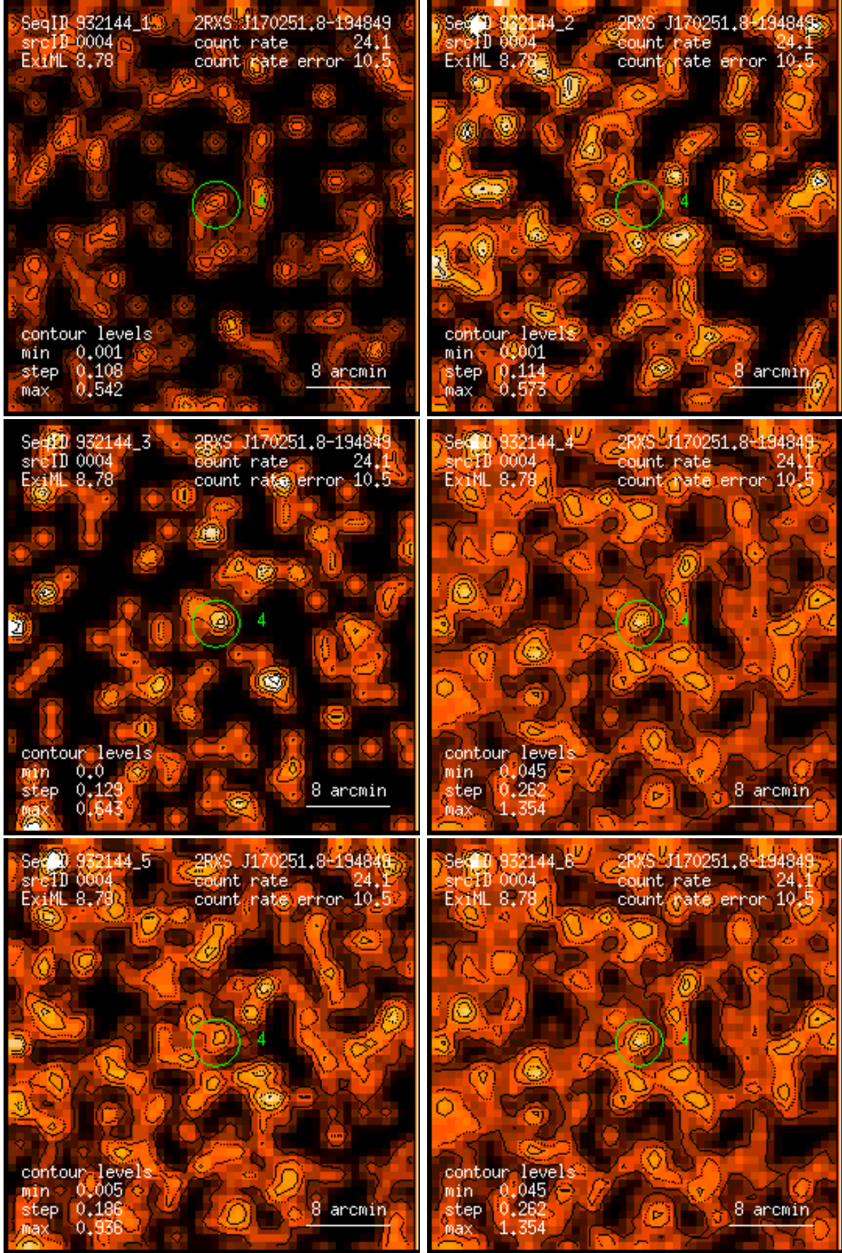
Figure 4: RASS 932144: detection 0004: band rate images, Gaussian filter: (1) PSPC channels 11 – 41, (2) 52 – 90, (3) 91 – 201, (4) 11 – 235, (5) 52 – 201, (6) 11 – 201. Broad band rates in counts/ks. Band rate contour levels in counts/ks/arcmin 2 .
