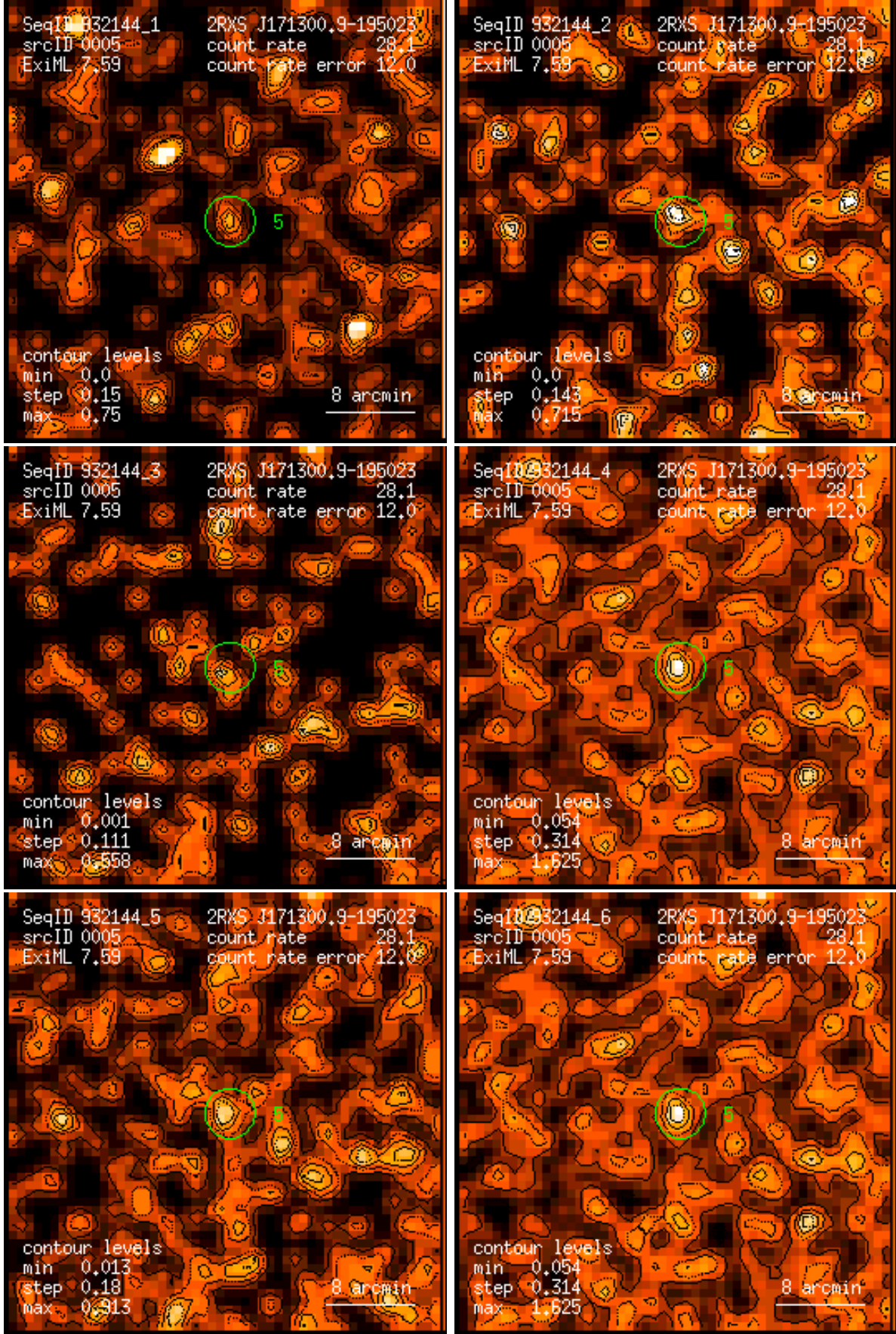
Figure 5: RASS 932144: detection 0005: band rate images, Gaussian filter: (1) PSPC channels 11 – 41, (2) 52 – 90, (3) 91 – 201, (4) 11 – 235, (5) 52 – 201, (6) 11 – 201. Broad band rates in counts/ks. Band rate contour levels in counts/ks/arcmin 2 .
